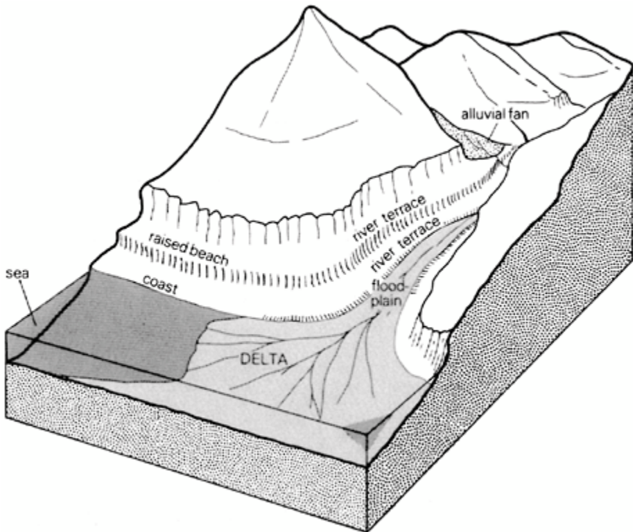
Figure 3.7 The mountain stream has deposited the coarser part of its load as an alluvial fan where the gradient changes suddenly at the plain. Deposition of finer sediment has taken place at the coast to form a delta. As the river winds towards the coast, it cuts a broad floodplain. The river terrace is an older floodplain, which is now well above the river bed.
