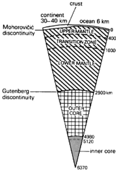
Figure 4.29 Layers of the Earth and major discontinuities.
