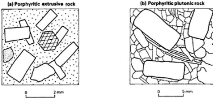
Figure 2.17 Porphyritic rocks.
