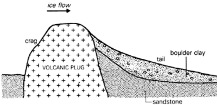
Figure 3.17 A vertical section across a crag and tail. On the left, a rock relatively resistant to glacial erosion (in this case the igneous rocks of a volcanic plug) is left protruding as a crag. It shelters softer sandstones in its lee from erosion by ice and they are left forming part of a streamlined 'tail' pointing in the direction of ice flow. The change of pressure at the base of the ice has left a thicker cover of boulder clay on the tail.
