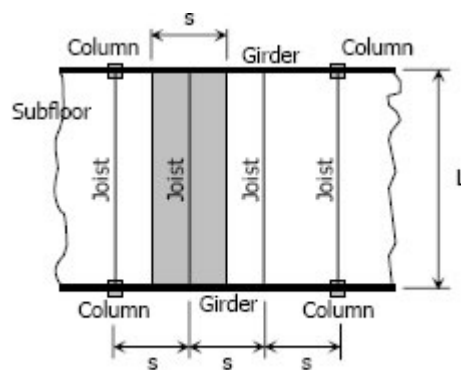
Typical Floor Framing Plan
