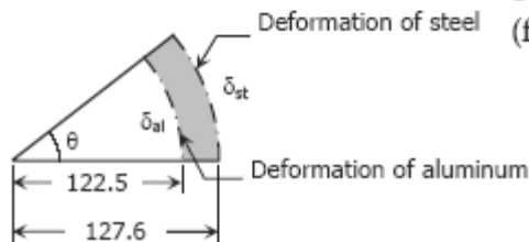
Geometric relation of deformations
