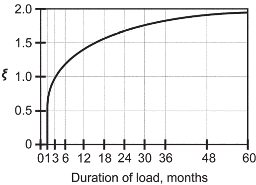
Fig. R24.2.4.1—Multipliers for time-dependent deflections.
