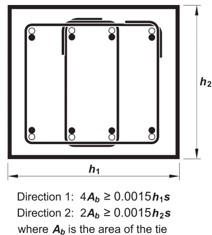
Fig. R10.7.5.2.1—Example of application of 10.7.5.2.1(a).
