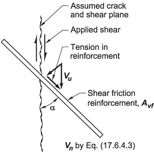
Fig. R22.9.4.3a—Tension in shear friction reinforcement.
