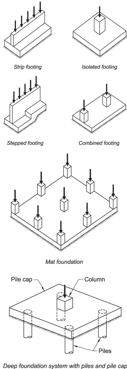
Fig. R13.1.1—Types of foundations.
