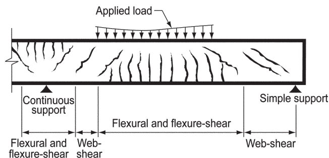
Fig. R22.5.8.3 —Types of cracking in concrete beams.
