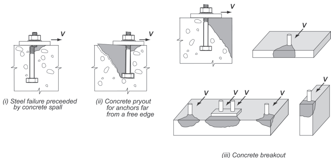
Fig. R17.3.1—Failure modes for anchors.
