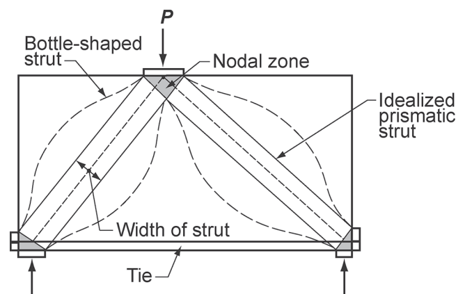
Fig. R23.2.1—Description of strut-and-tie model.
