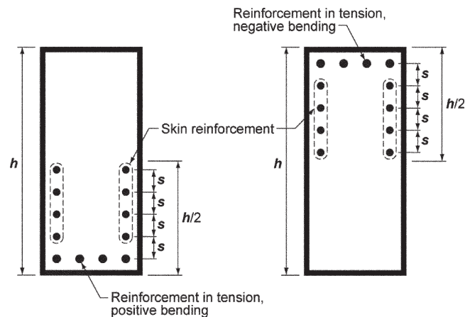
Fig. R9.7.2.3 —Skin reinforcement for beams and joists with h > 36 \text{ in.}
