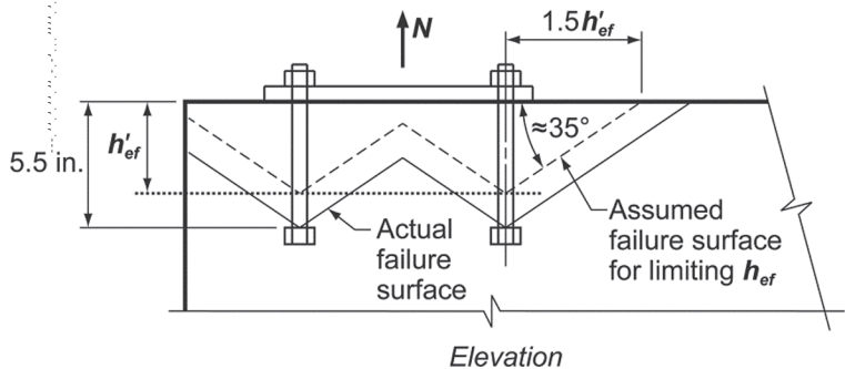
Fig. R17.4.2.3—Example of tension where anchors are located in narrow members.
