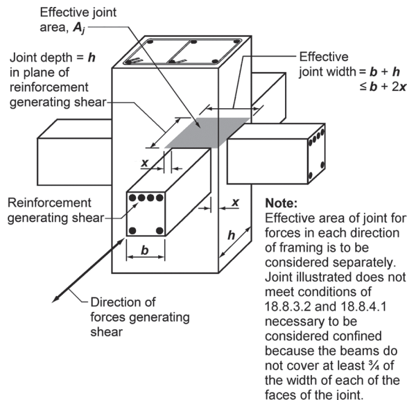
Fig. R18.8.4—Effective joint area.
