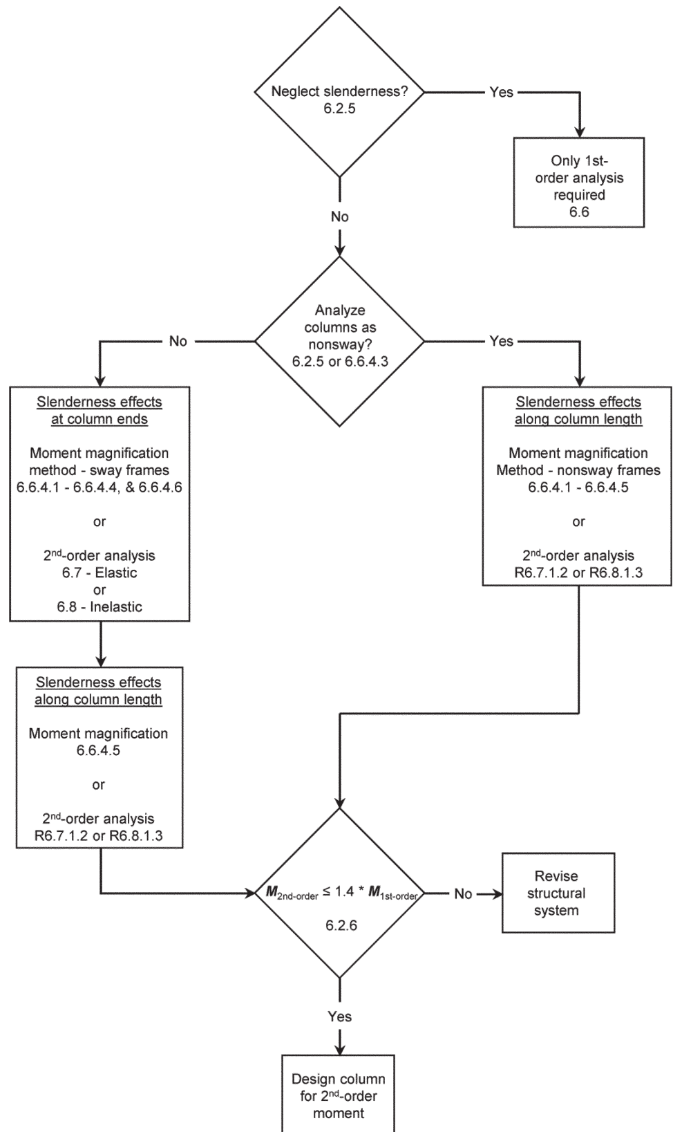
Fig. R6.2.6 —Flowchart for determining column slenderness effects.
