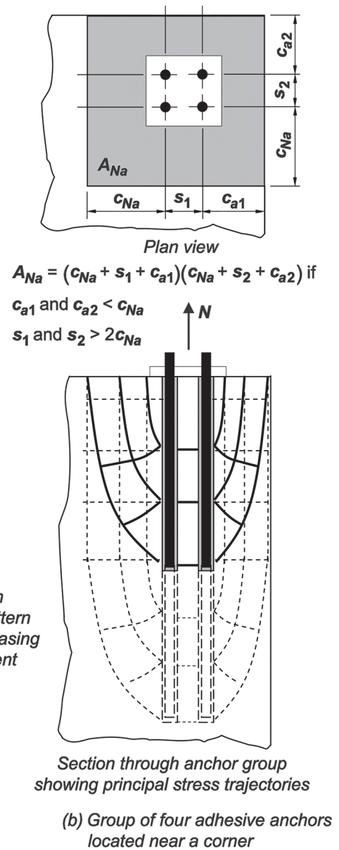
Fig. R17.4.5.1 —Calculation of influence areas A_{Na0} and A_{Na} .
