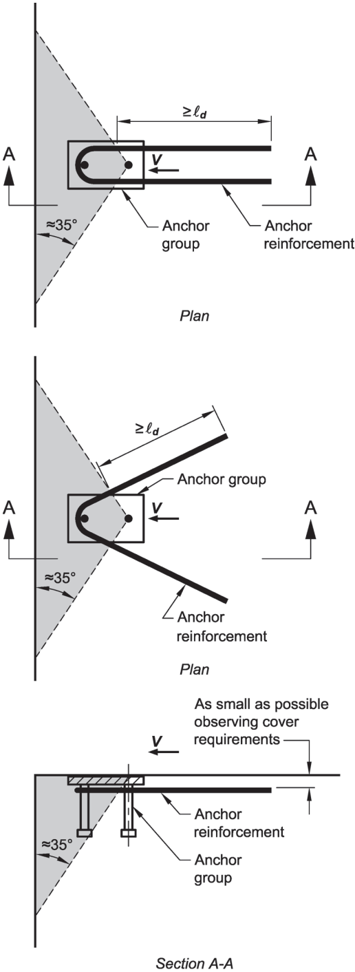
Fig. R17.5.2.9a—Hairpin anchor reinforcement for shear.
