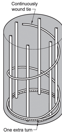
Fig. R25.7.2.3b —Continuous tie anchorage.
