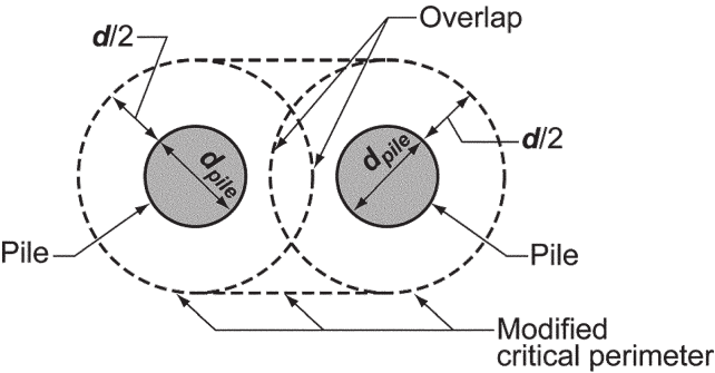
Fig. R13.2.7.2—Modified critical perimeter for shear with overlapping critical perimeters.
