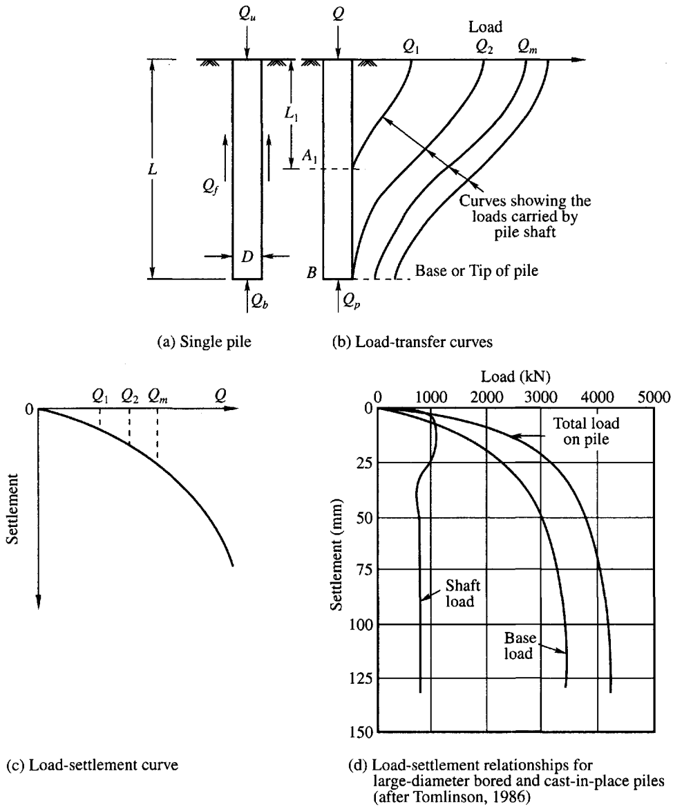
Figure 15.4 Load transfer mechanism
