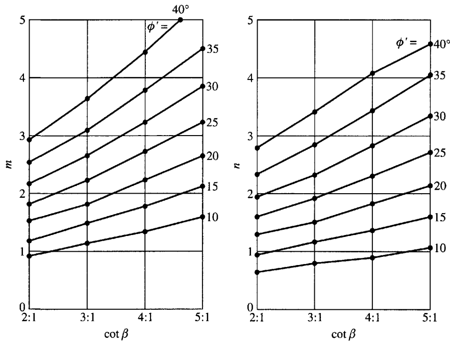
Figure B.5 Stability coefficients m and n for c'/\gamma H = 0.05 and n_d = 1.25 (Bishop and Morgenstern, 1960)
