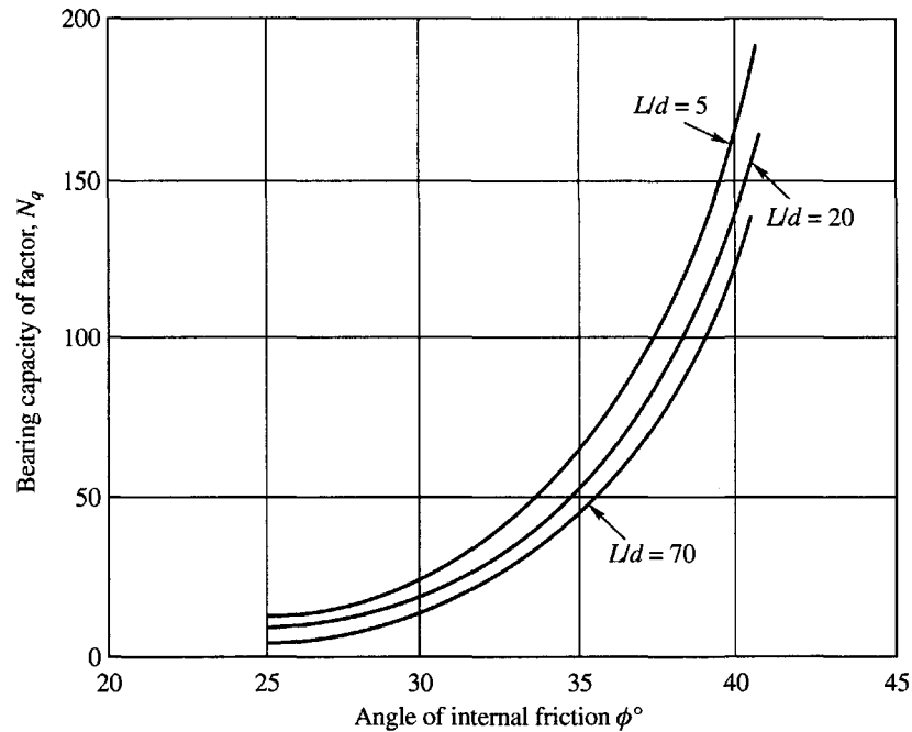
Figure 15.9 Berezantsev's bearing capacity factor, N_q (after Tomlinson, 1986)
