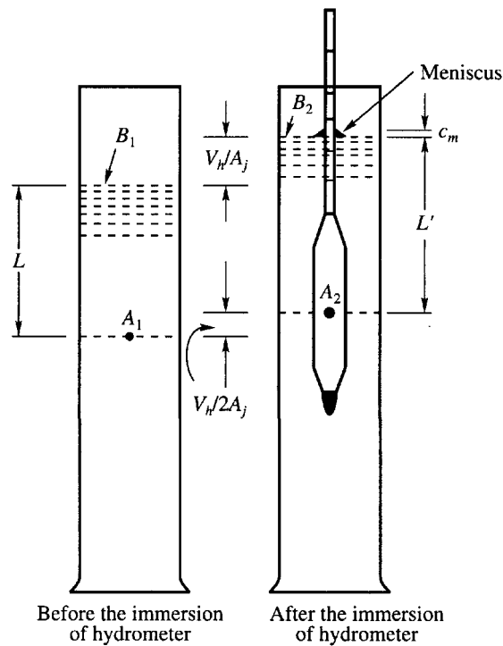
Figure 3.6 Immersion correction
