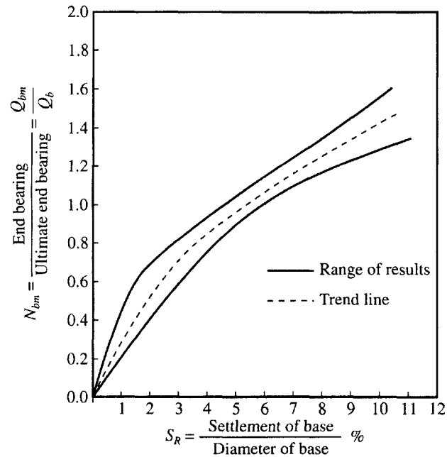
Figure 17.21 Normalized base load transfer for drilled shaft in cohesionless soil (O'Neill and Reese, 1999)
