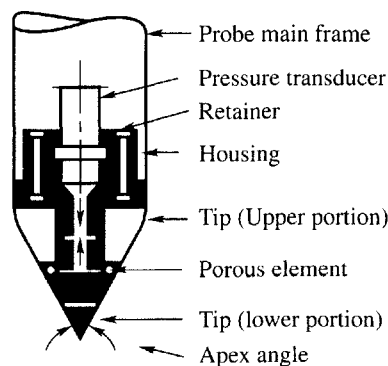
Figure 9.13 Details of 60°/10 cm 2 piezocone
