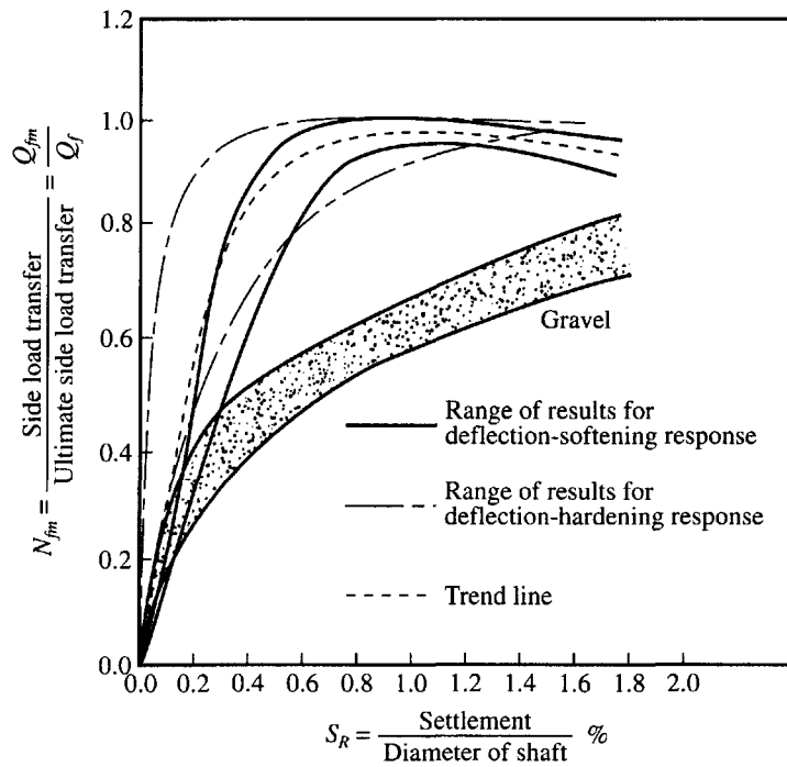
Figure 17.20 Normalized side load transfer for drilled shaft in cohesionless soil (O'Neill and Reese, 1999)
