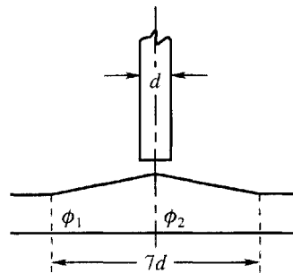
Figure 15.7 The effect of driving a pile on \phi
