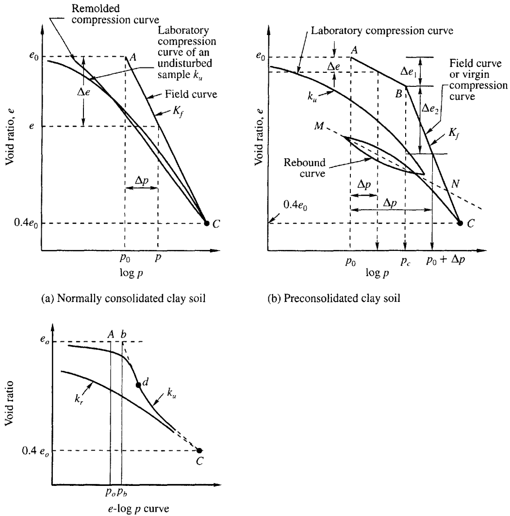
(c) Typical e-log p curve for an undisturbed sample of clay of high sensitivity (Peck et al., 1974)
