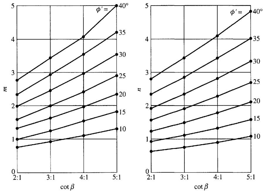
Figure B.3 Stability coefficients m and n for c'/\gamma H = 0.025 and n_d = 1.25 (Bishop and Morgenstern, 1960)
