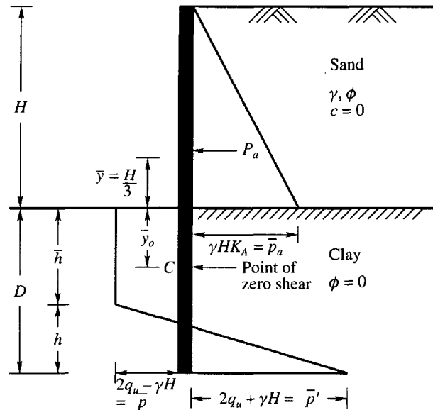
Figure 20.11 Sheet pile wall embedded in clay with sand backfill.
