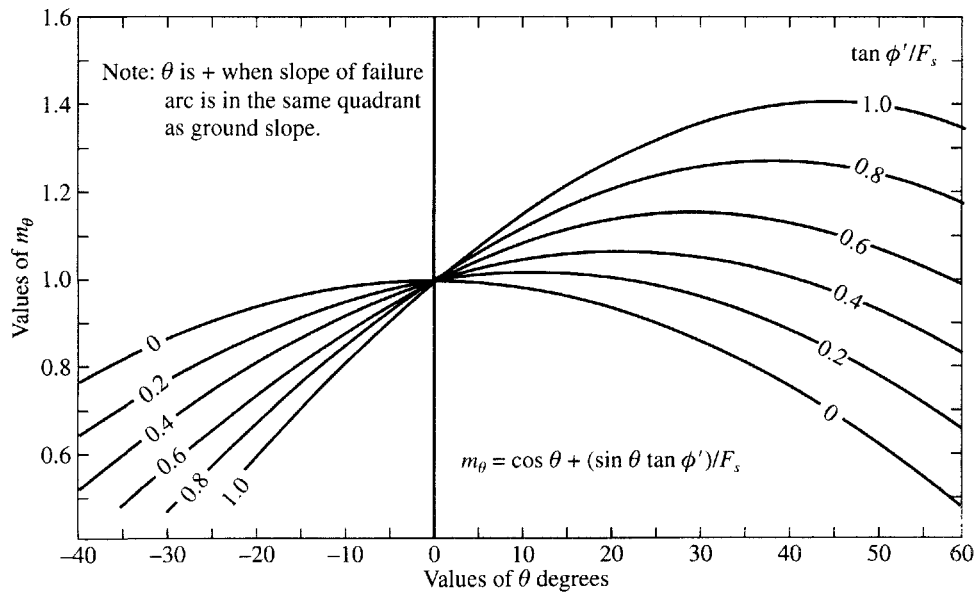
Figure 10.24 Values of m_\theta (after Janbu et al., 1956)
