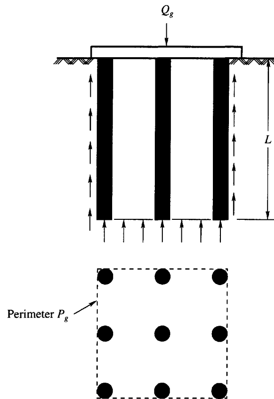
Figure 15.27 Block failure of a pile group in clay soil
