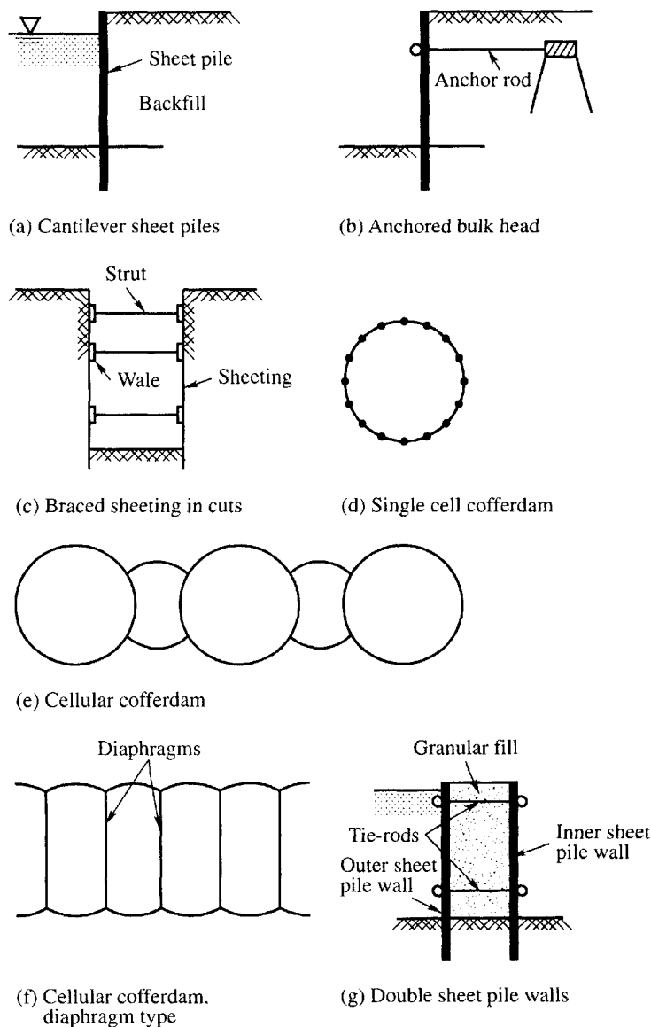
Figure 20.4 Use of sheet piles
