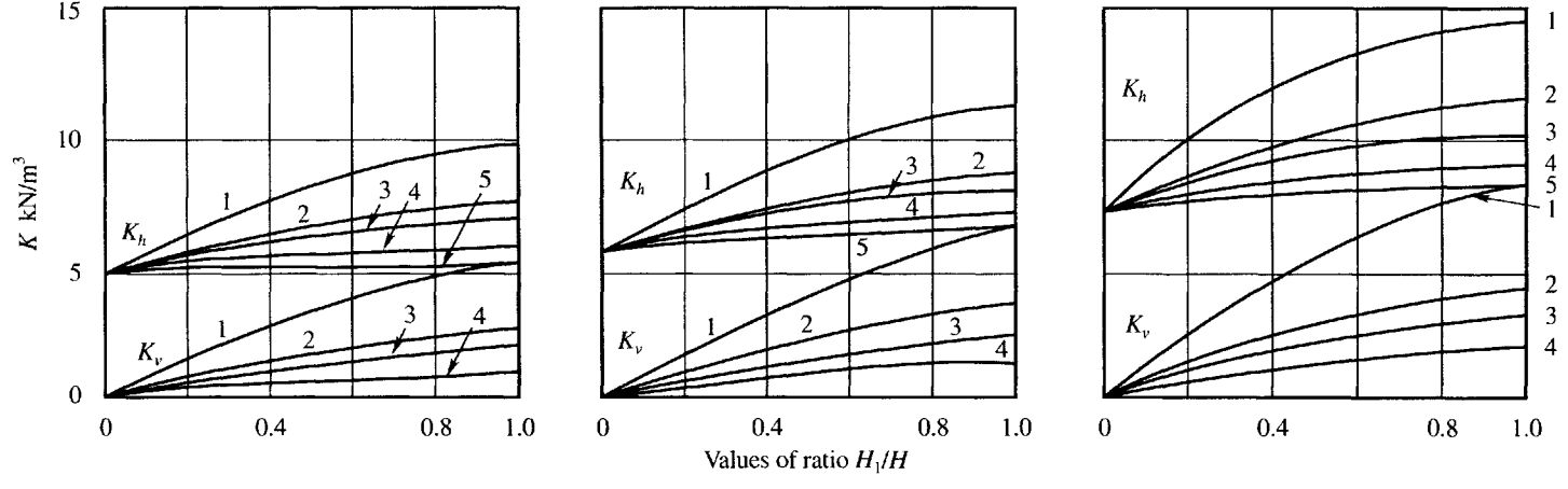
Figure 19.5 Chart for estimating pressure of backfill against retaining walls supporting backfills with a surface that slopes upward from the crest of the wall for limited distance and then becomes horizontal. (Terzaghi et al., 1996)
