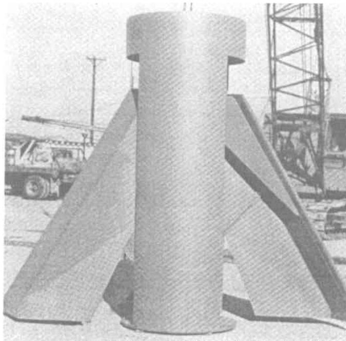
Figure 17.5 A 30° underreamer with blade cutters for soils that can be cut readily (Source: Woodward et al., 1972)
