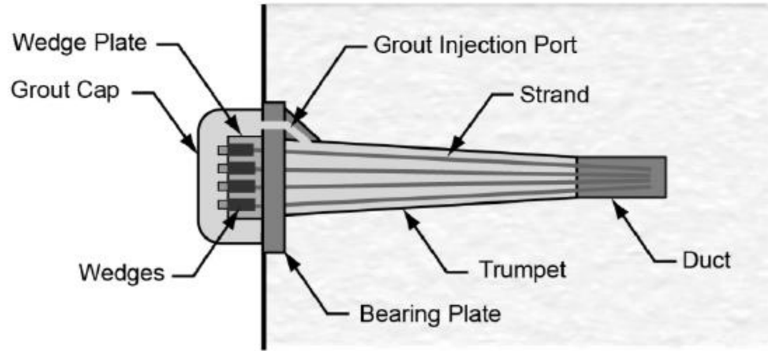
Normal Anchorage (Plate Anchorage Shown)
