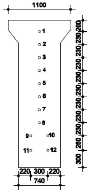
SECTION AT END (SHOWING LOCATION OF CABLES)
