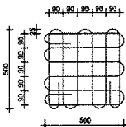
Y8 MESH REINF. ABOVE BEARINGS
