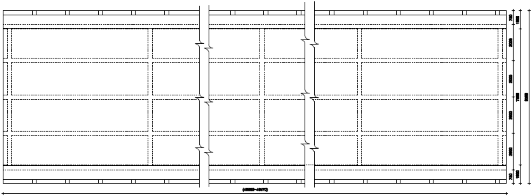
TYPICAL BRIDGE DECK PLAN
