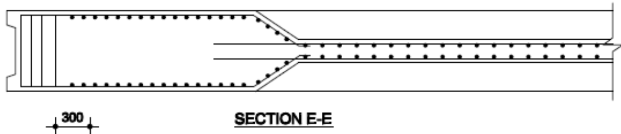
SECTION AT END (SHOWING LOCATION OF CABLES)
