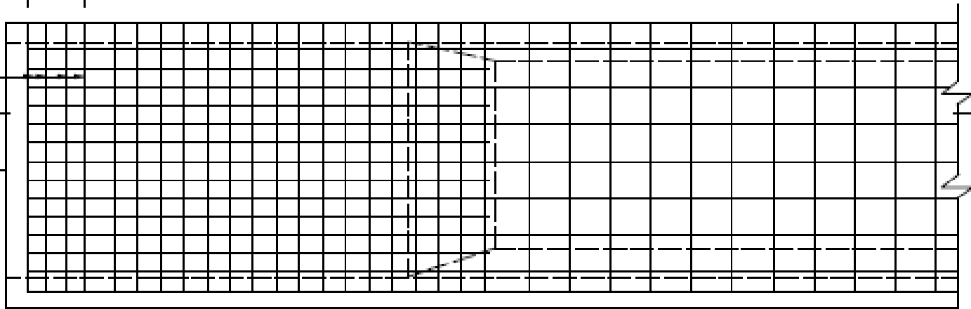
DETAIL OF END BLOCK
