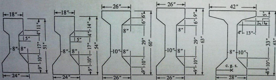
FIGURE 7.34 Standard I-beams used by the Pennsylvania Department of Transportation [PennDOT, 1993b].
