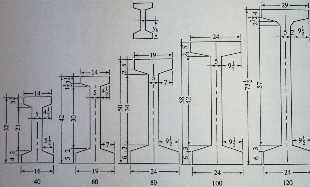
FIGURE 7.32 Washington State standard I-girders.
