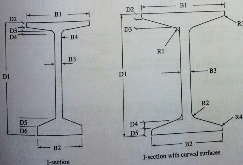
FIGURE 7.31 New I-girder series developed by Nebraska University for the Nebraska Department of Roads, to be used
