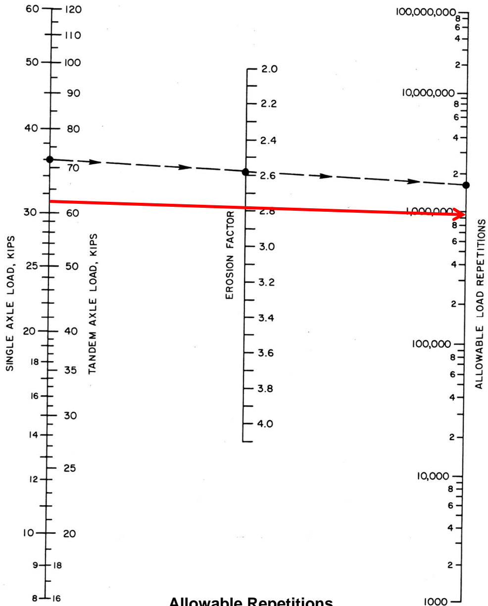
Allowable Repetitions No Concrete Shoulder
