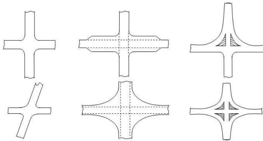
Unchannelized Cross
