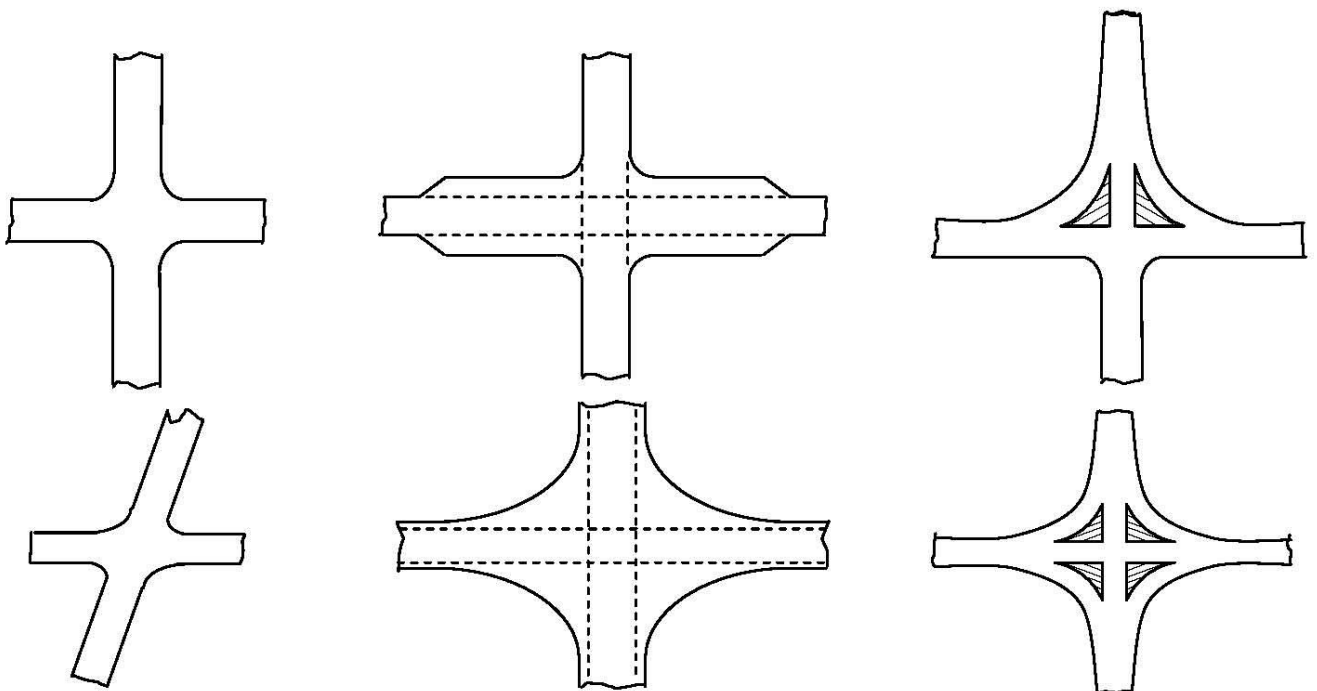
Unchannelized Cross
