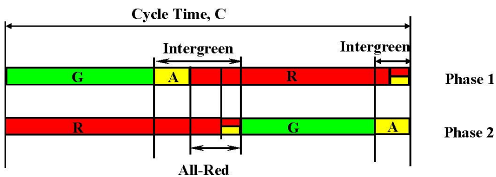
EXAMPLE OF INTERGREEN & ALL-RED PERIODS
