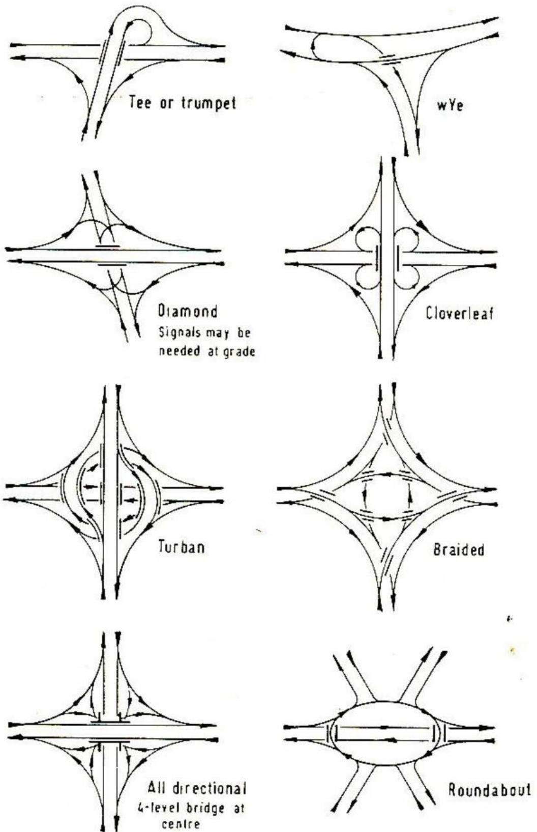
Fig. 6.26. Diagrammatic examples of some basic traffic movements at interchanges
