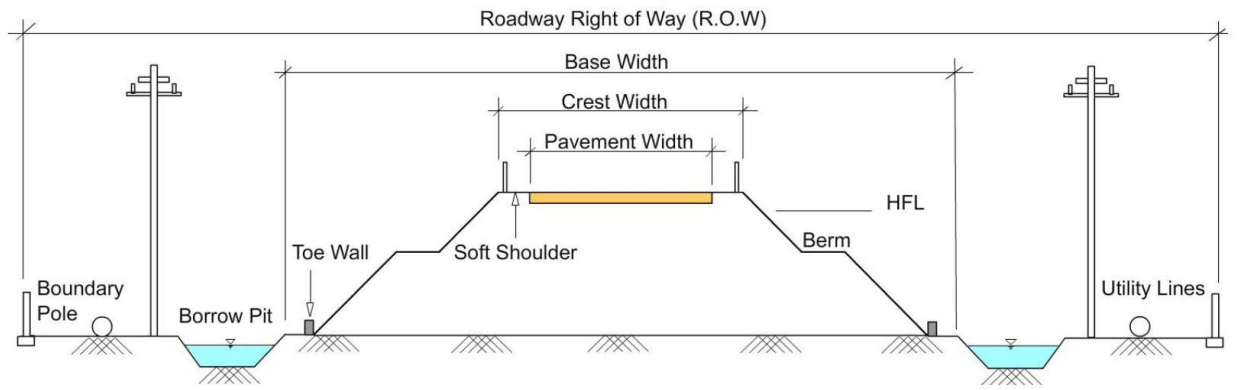
Typical Cross-Section of Highway Embankment
