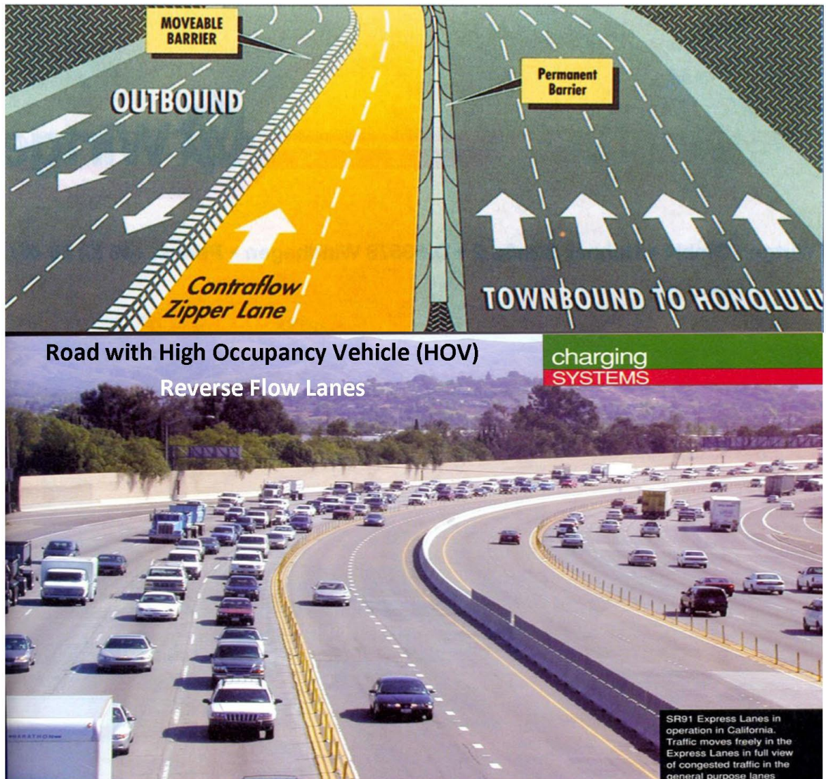
Figure 1: Trinary Road Concept
