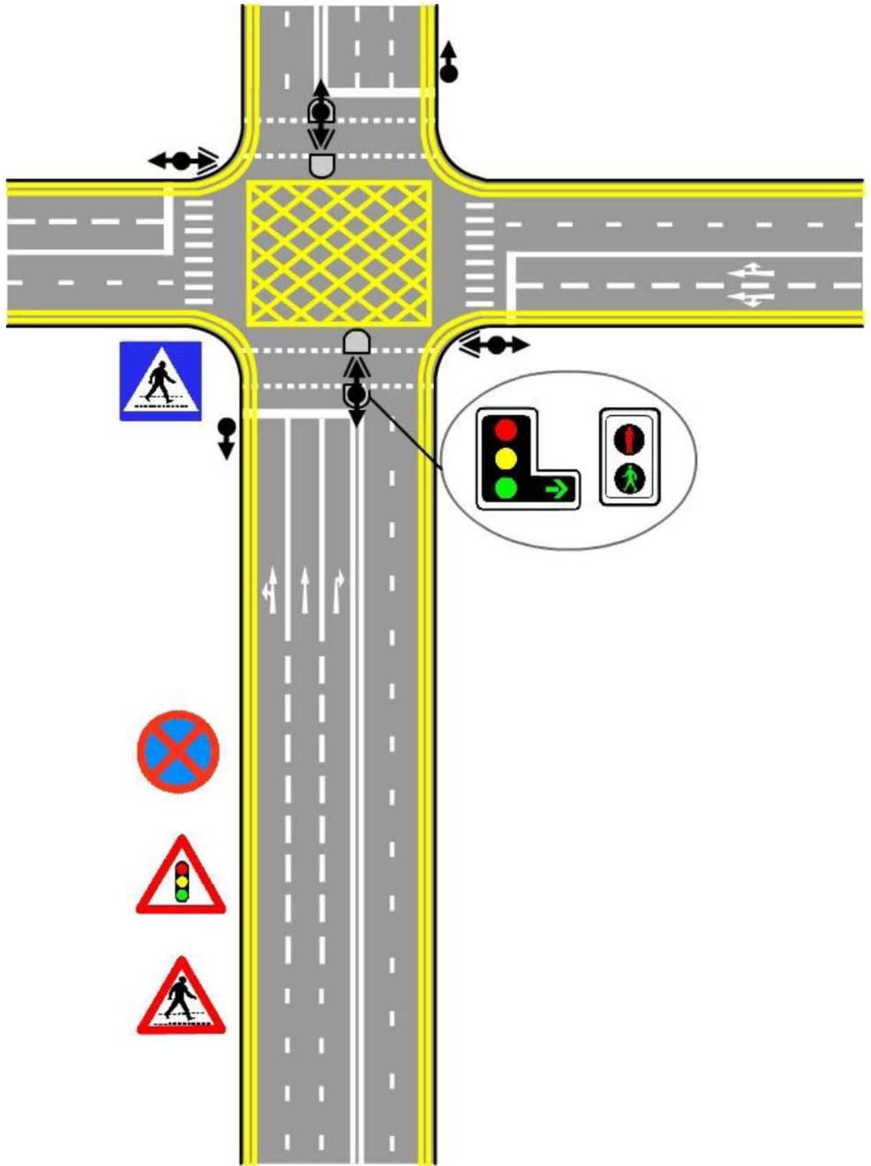
DIFFERENT ROAD SIGNS AND MARKINGS
