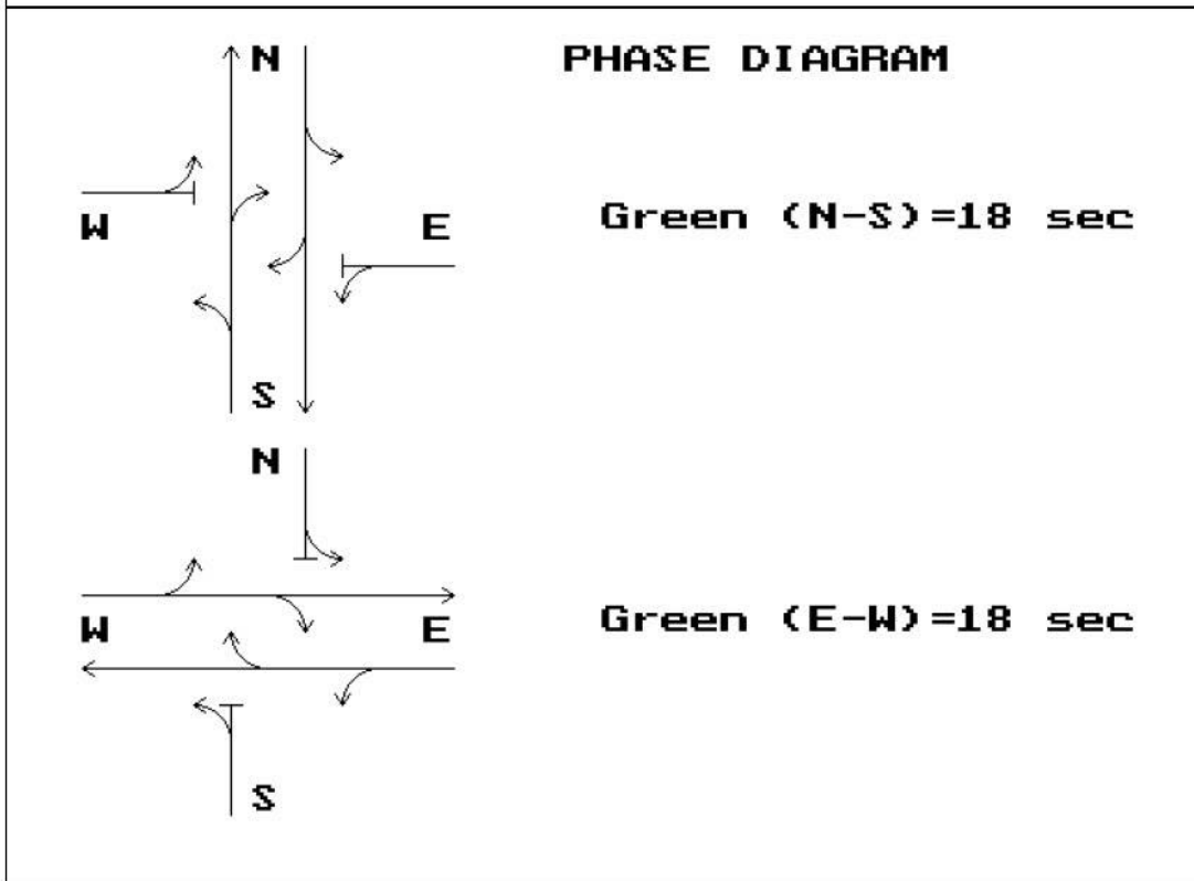
TRAFFIC MOVEMENTS IN A TWO-PHASE SYSTEM
