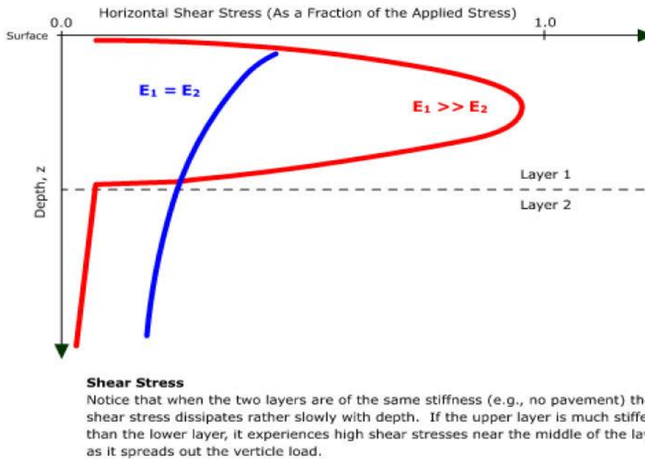
Figure 1: Typical Two-Layer Flexible Pavement Stresses as Calculated by a Two-Dimensional Linear Elastic Model.
