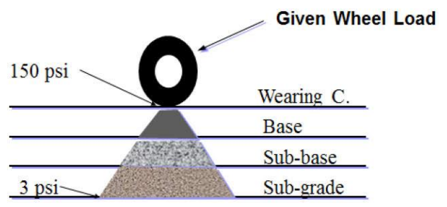
Load Distribution in Flexible Pavements
