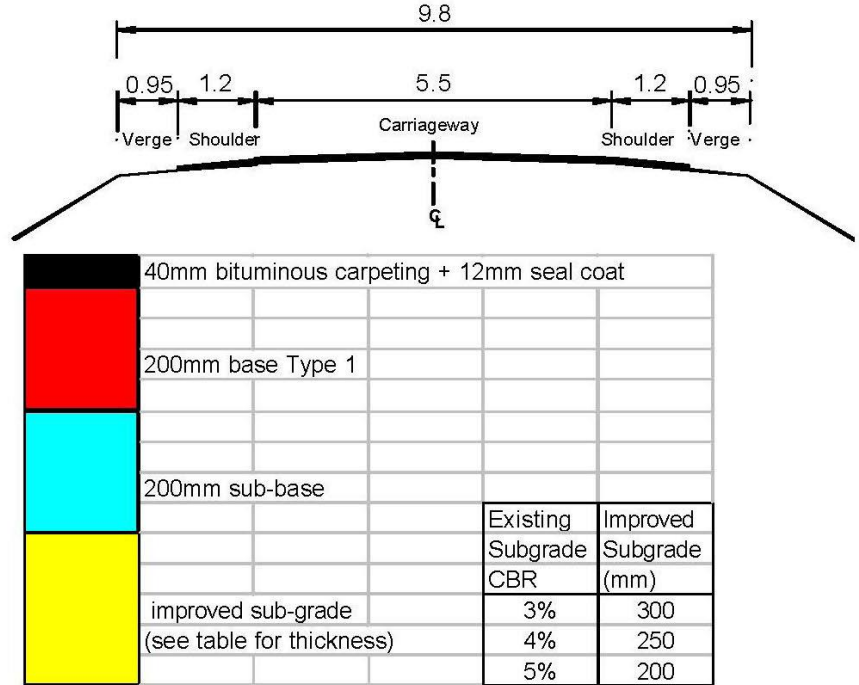
Type 5: 5.5m Carriageway
