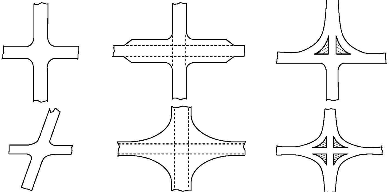
Unchannelized Cross
