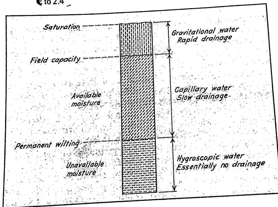
Fig: Classes and soil-water availability to plants and drainage characteristics
