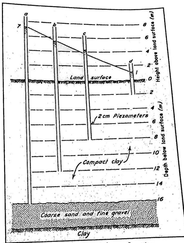
Fig: Flow of confined ground water
