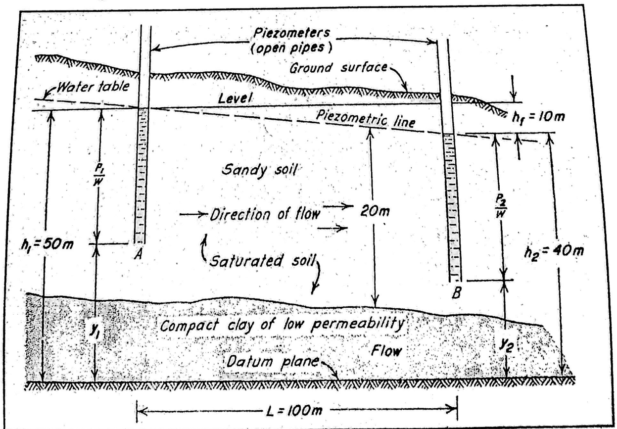
Fig: Flow of unconfined ground water
