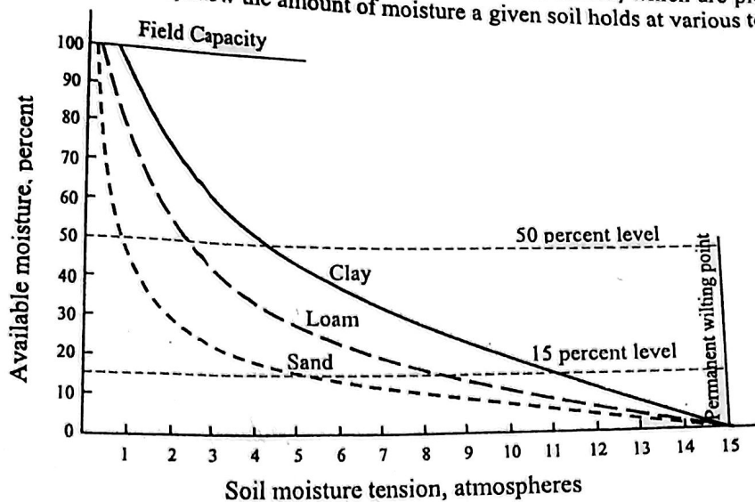
Fig: Typical moisture characteristics curves
