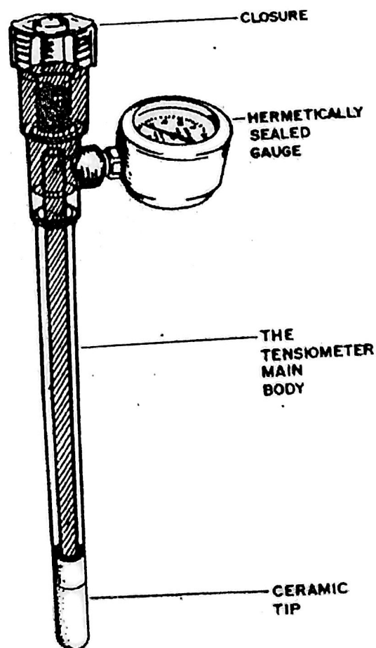
Fig: The essential parts of a tensiometer
