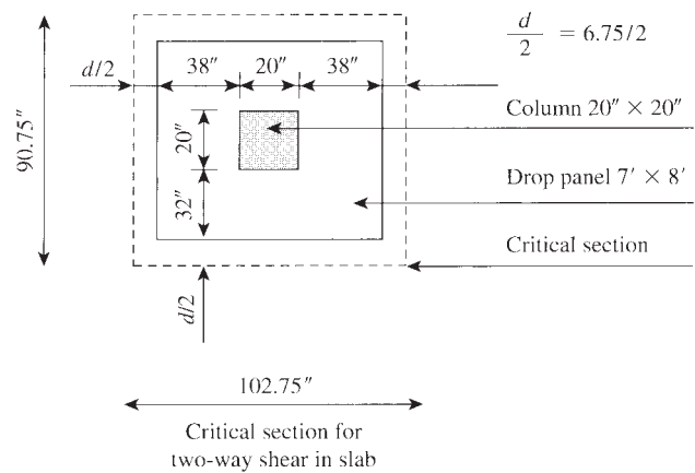
Figure 17.32 Example 17.11: Flat slab with drop panel.
