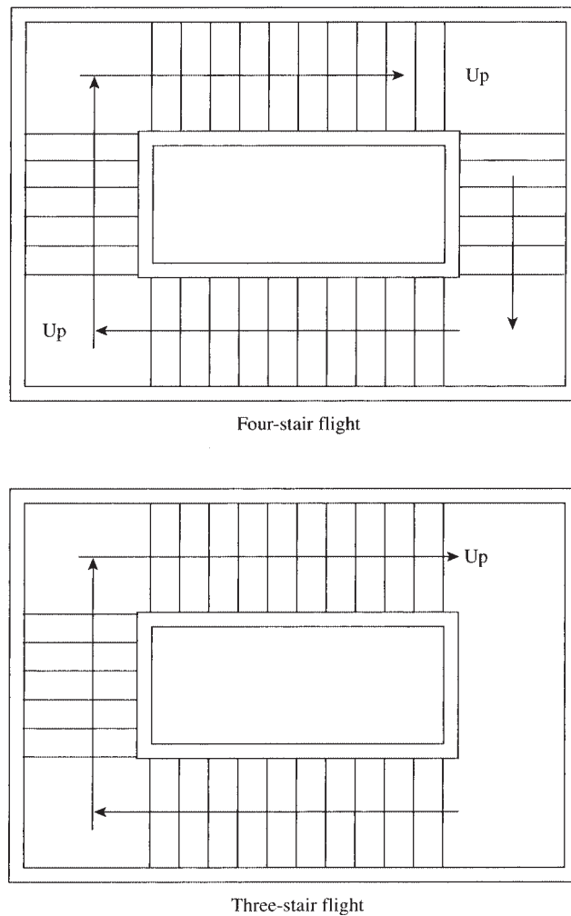
Figure 18.6 Three- and four-stair flights.
