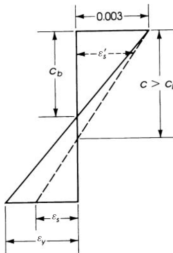
Figure 11.9 Strain diagram when compression controls. When \varepsilon_s < \varepsilon_y , c > c_b and \varepsilon'_s \geq \varepsilon_y .
