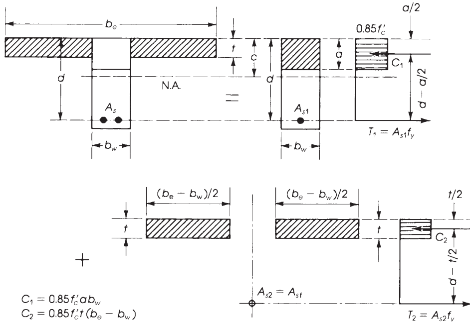
Figure 3.32 T-section analysis.
