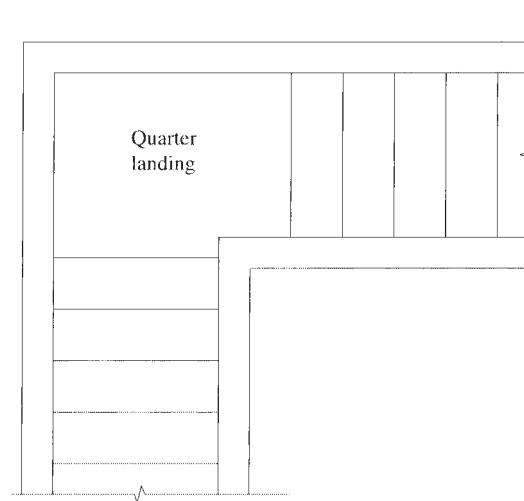
Figure 18.4 Quarter-turn staircase.
