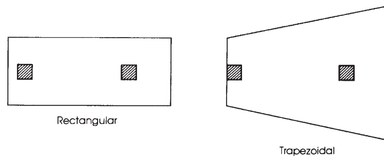
Figure 13.23 Combined footings.
