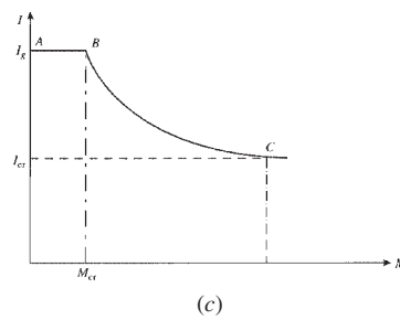
Figure 6.2 (a) Experimental and theoretical load–deflection curves for a beam of the section and load illustrated, (b) deflection of a reinforced concrete beam, and (c) variation of beam moment of inertia, I , with an increase in moment ( E = \text{const} ). BC is a transition curve between I_g and I_{cr} .
