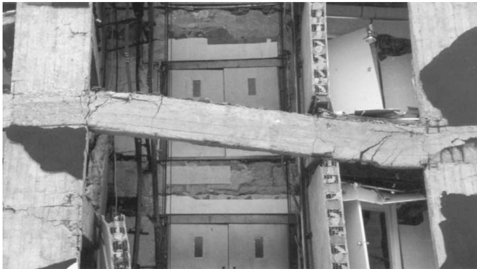
Strong column–weak beam connection. Courtesy of Murat Saatcioglu and John Gardner.
