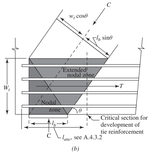
Figure 8.7 Extended nodal zones and hydrostatic nodes [1]: (a) one layer of steel, (b) distributed steel, (c) geometry, (d) tension force anchored by a plate, and (e) tension force anchored by bond. Courtesy of ACI 3-18-11.
