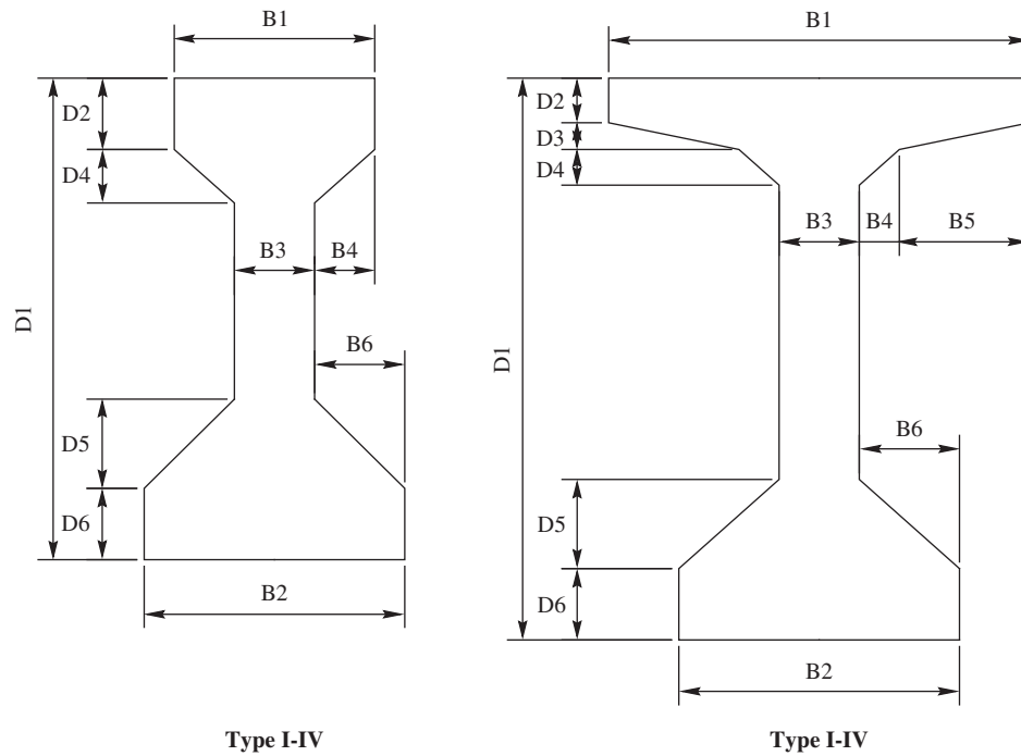
Figure 22.3 Cross section of AASHTO I-beams.
