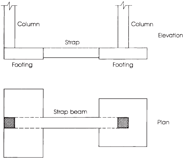
Figure 13.4 Strap footing.
