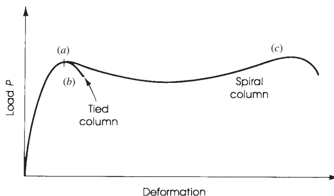
Figure 10.2 Behavior of tied and spiral columns.
