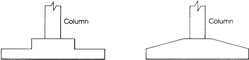
Figure 13.2 Single footing.
