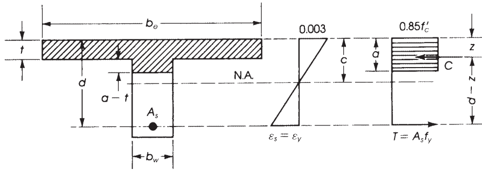
Figure 3.31 T-section behavior.
