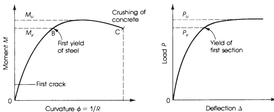
Figure 16.21 Yielding behavior of an underreinforced concrete beam.
