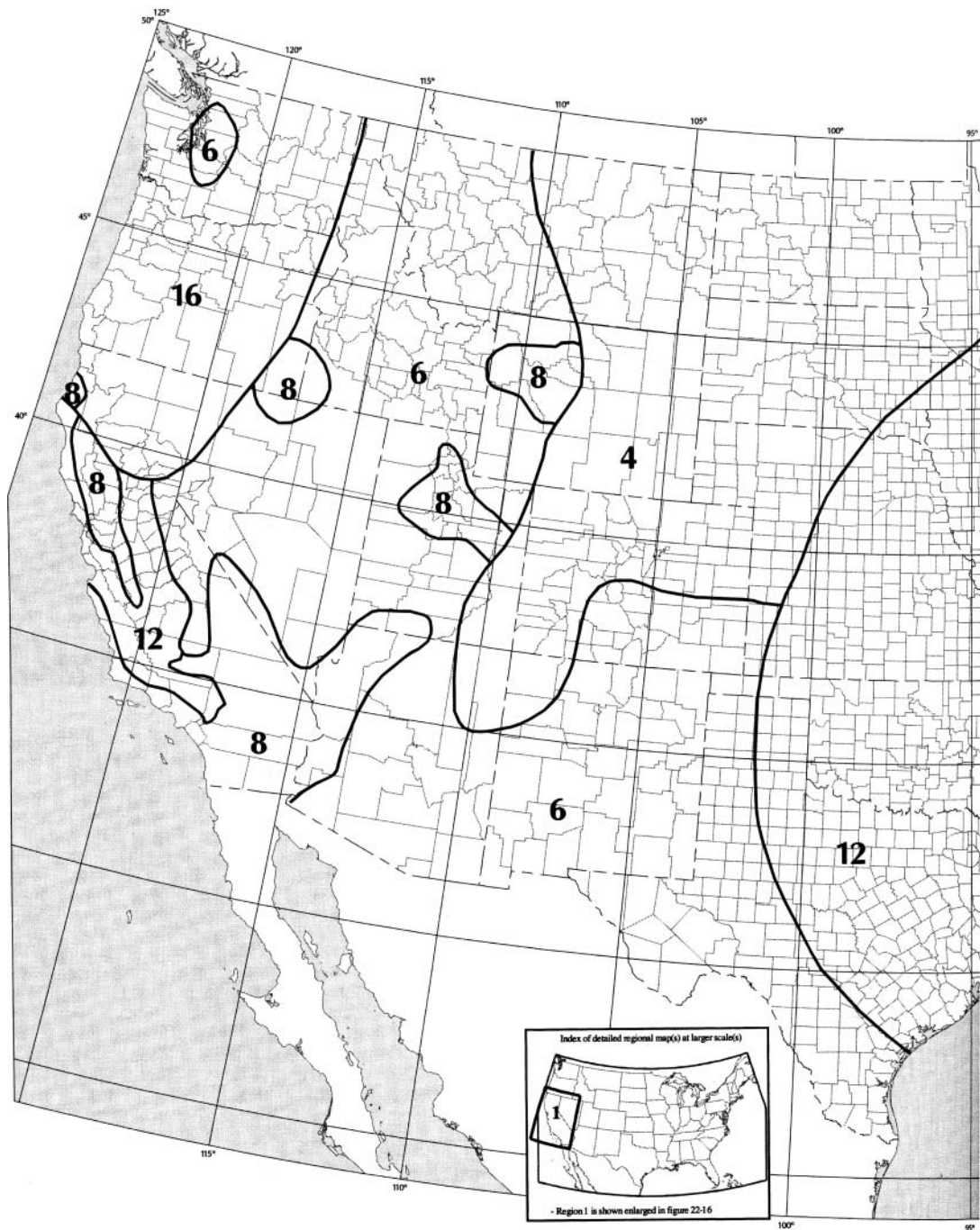
Figure 20.2a Long-period transition period, T_L (sec), for the conterminous United States. Source: ASCE 7-10 Minimum Design Loads for Buildings and Other Structures , 2010. With permission from ASCE.
