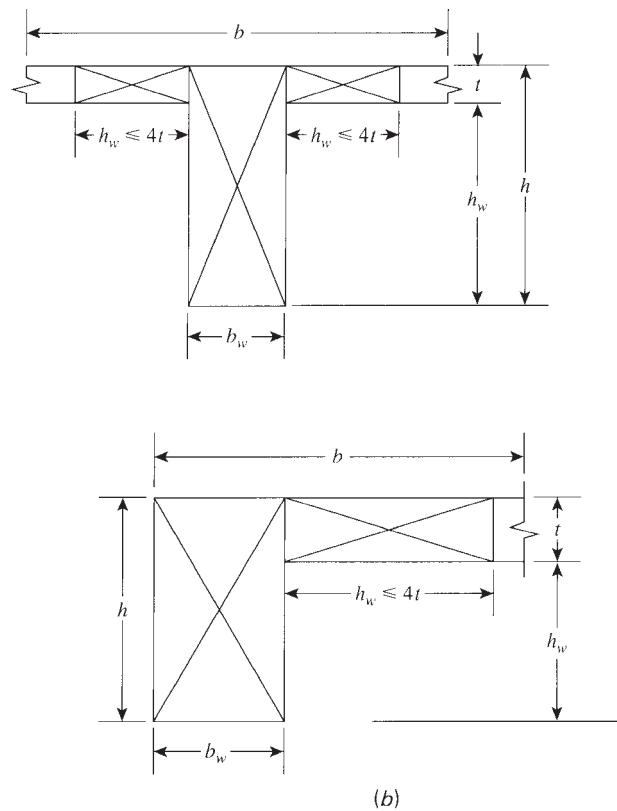
Figure 15.11 (a) Torsional geometric parameters and (b) effective flange width for T- and L-sections and component rectangles.
