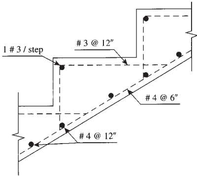
(e) Reinforcement details.
