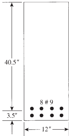
Figure 6.16 Skin reinforcement.
