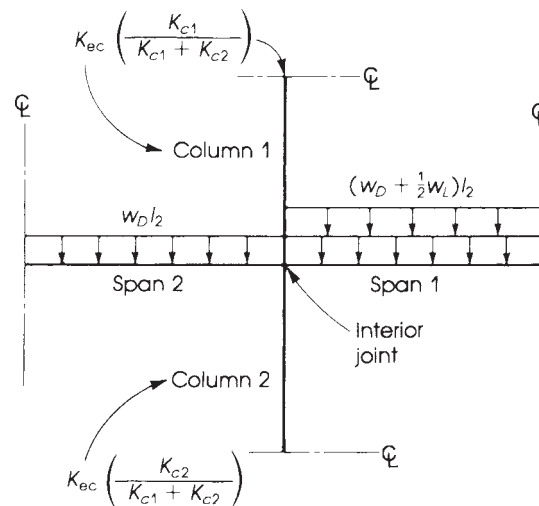
Figure 17.24 Interior column loading.
