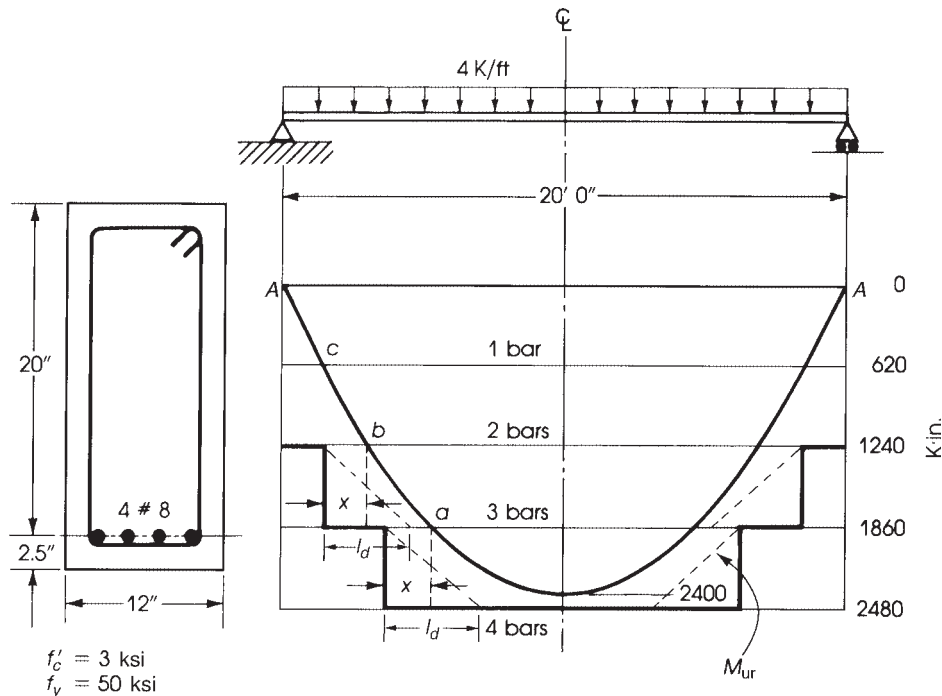
Figure 7.13 Moment–resistance diagram.
