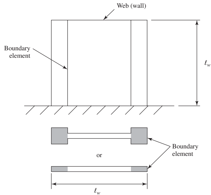
Figure 20.25 Boundary elements of structural wall.
