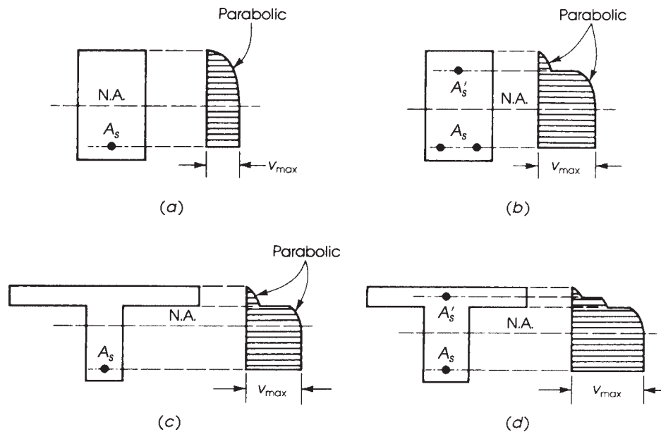
Figure 5.3 Distribution of shear stresses in reinforced concrete beams: (a) singly reinforced, (b) doubly reinforced, (c) T-section, and (d) T-section with compression steel.
