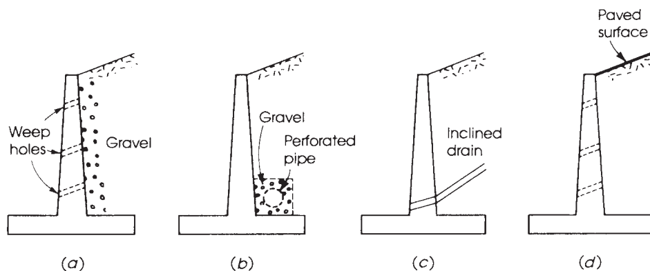
Figure 14.9 Drainage systems.
