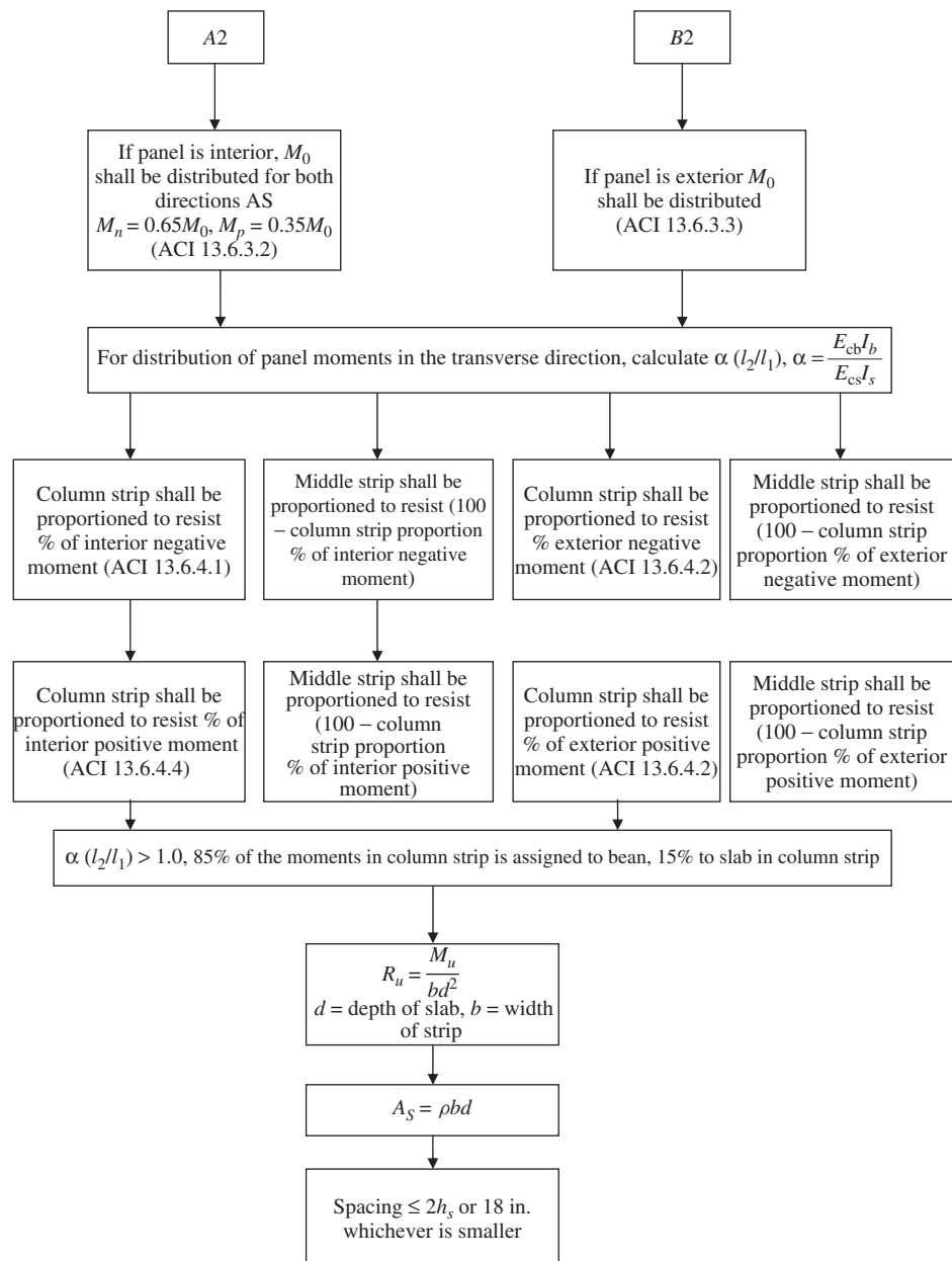
Flowchart 23.13e Two-way slab — DDM.
