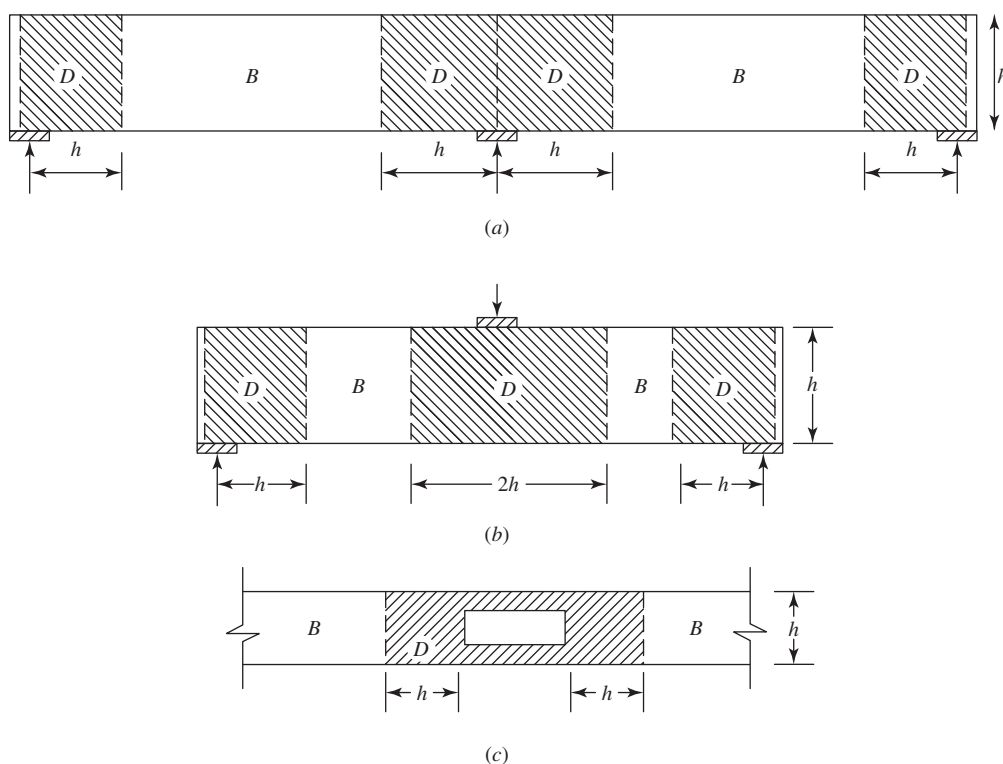
Figure 8.1 D - and B -regions in beam. (a) continuous beam, (b) beam with concentrated load, and (c) beam with an opening [1]. Courtesy of ACI 318.
