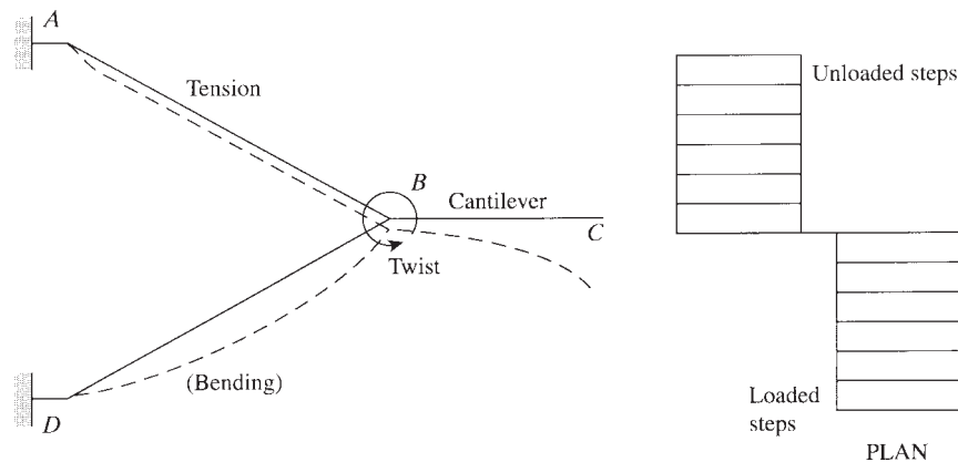
Figure 18.12 Case 2, DBC loaded.
