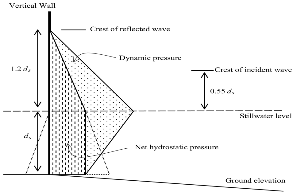
Figure 6.2.32 Normally incident breaking wave pressures against a vertical wall (still water level equal on both sides of wall)
