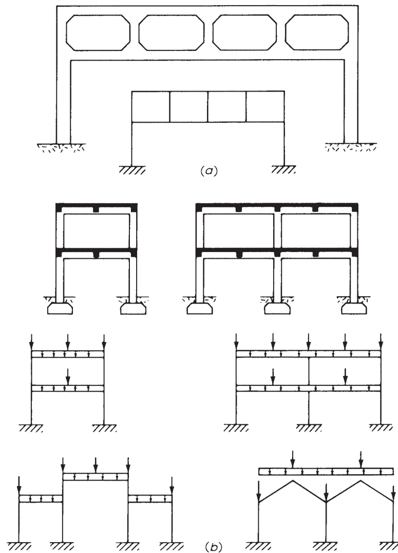
Figure 16.12 (a) Vierendeel girder and (b) statically indeterminate frames.
