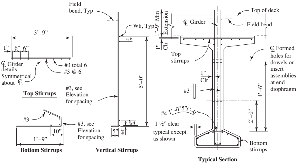
Figure 22.17 Girder reinforcement details.
