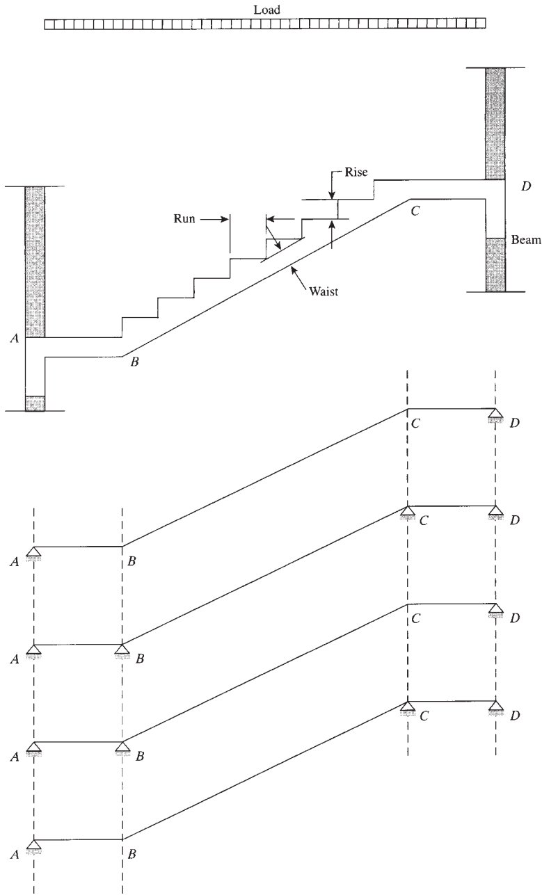
Figure 18.2 Supporting systems of one flight.
