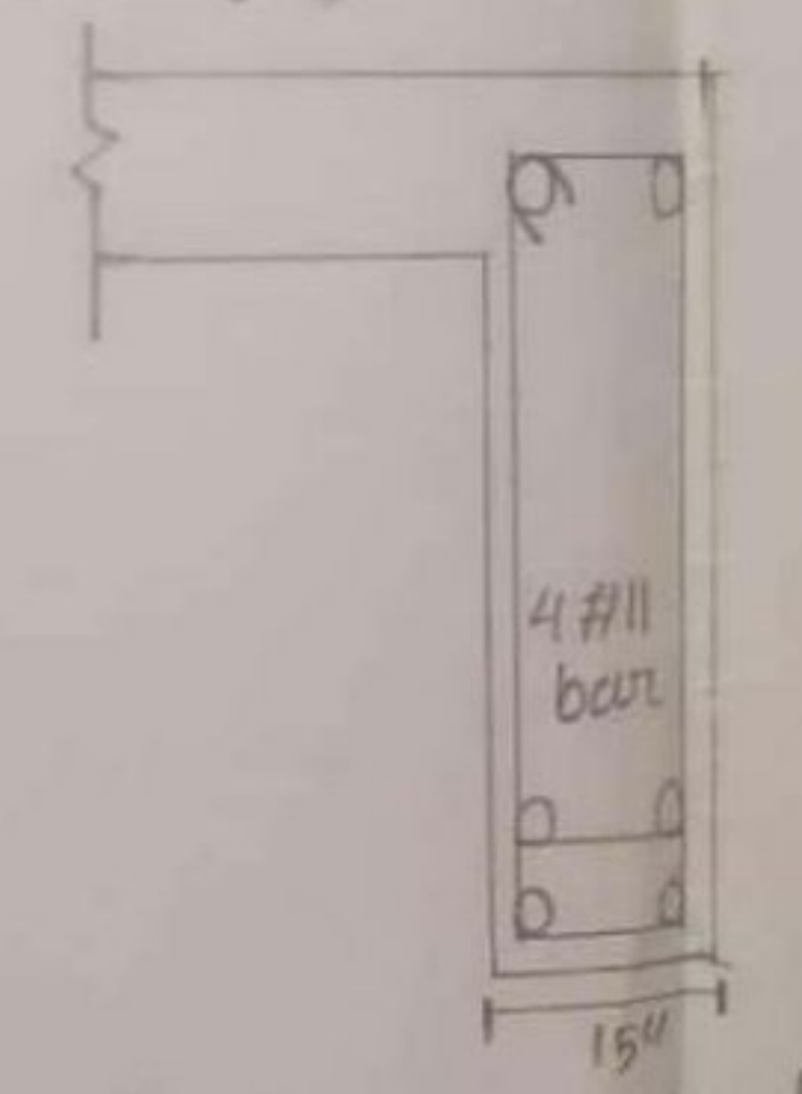
Fig: Reinforcement details at section 4-4
