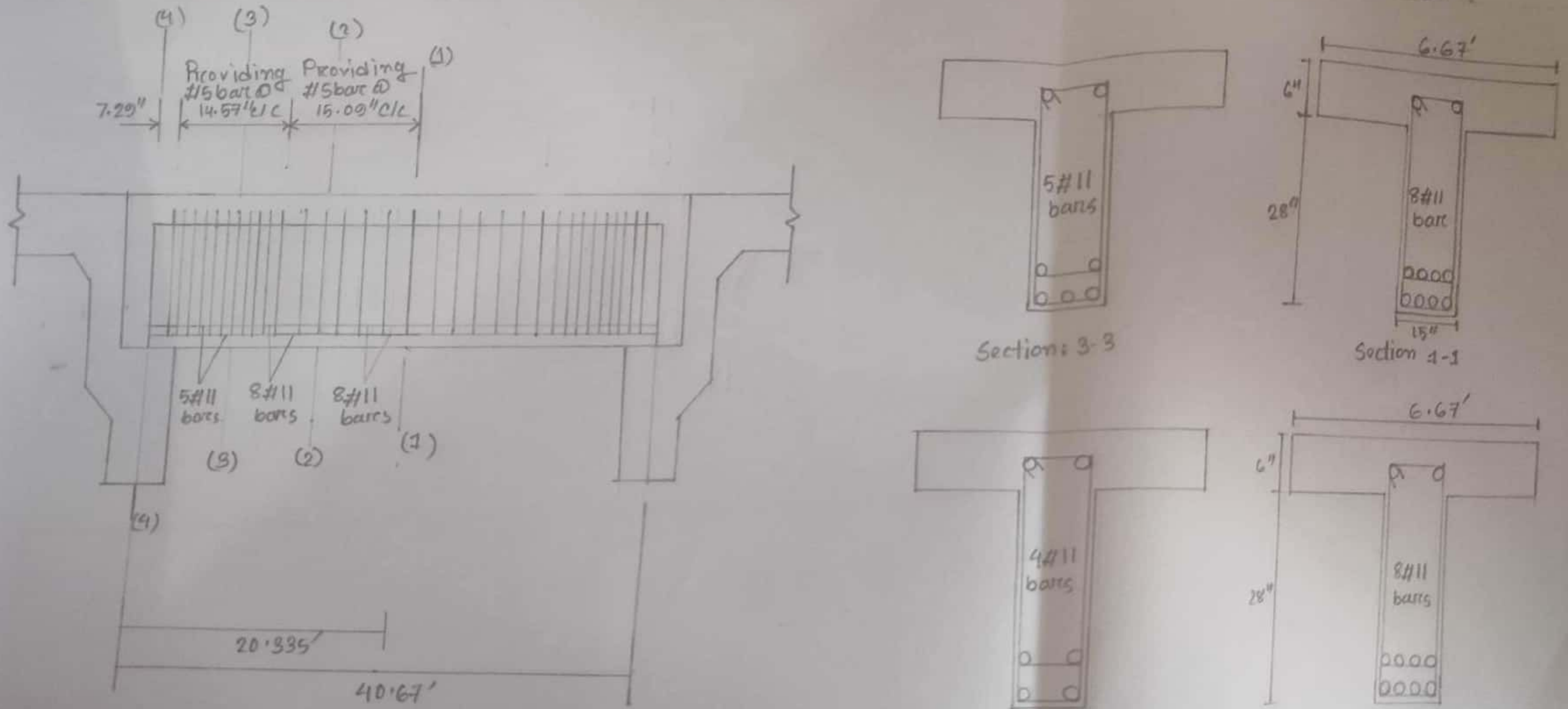
Fig: Reinforcement details of interior girder
