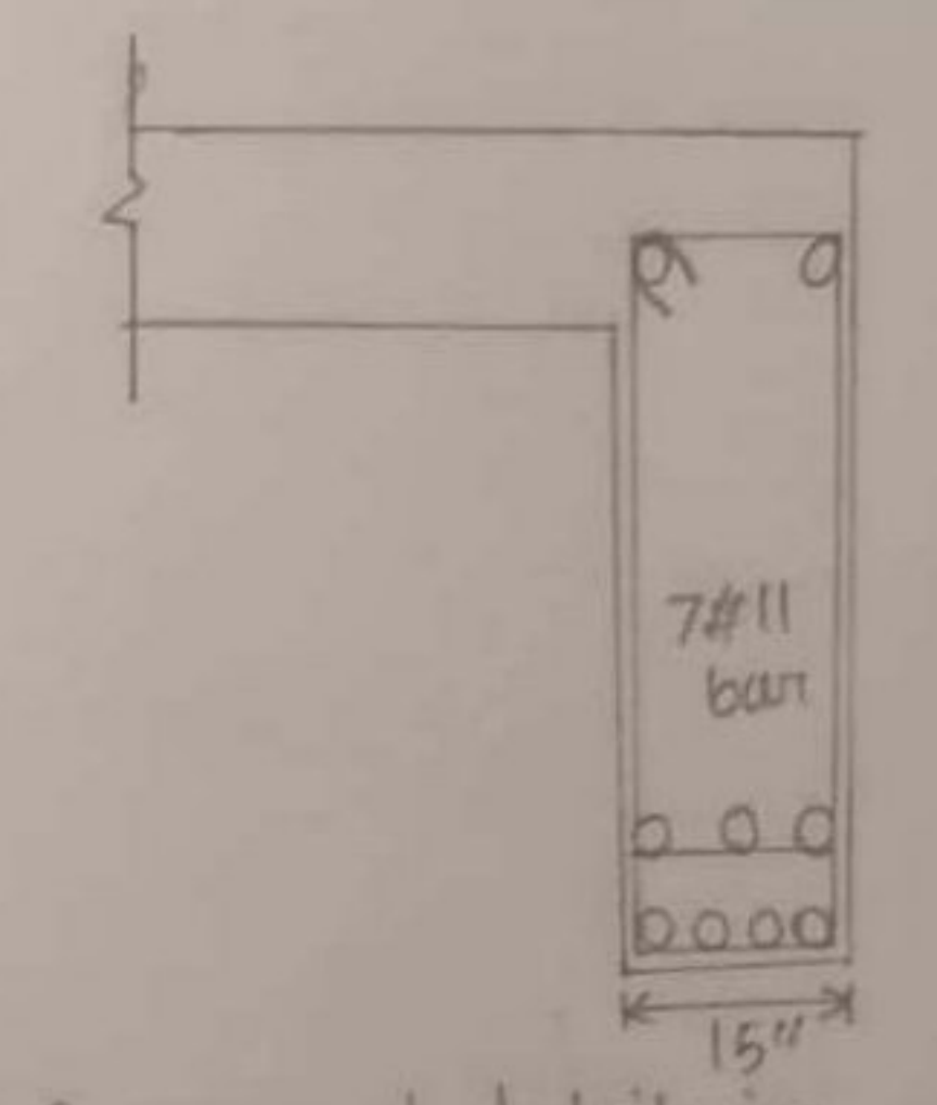
Fig: Reinforcement details in transverse section of Exterior girder at section 2-2
