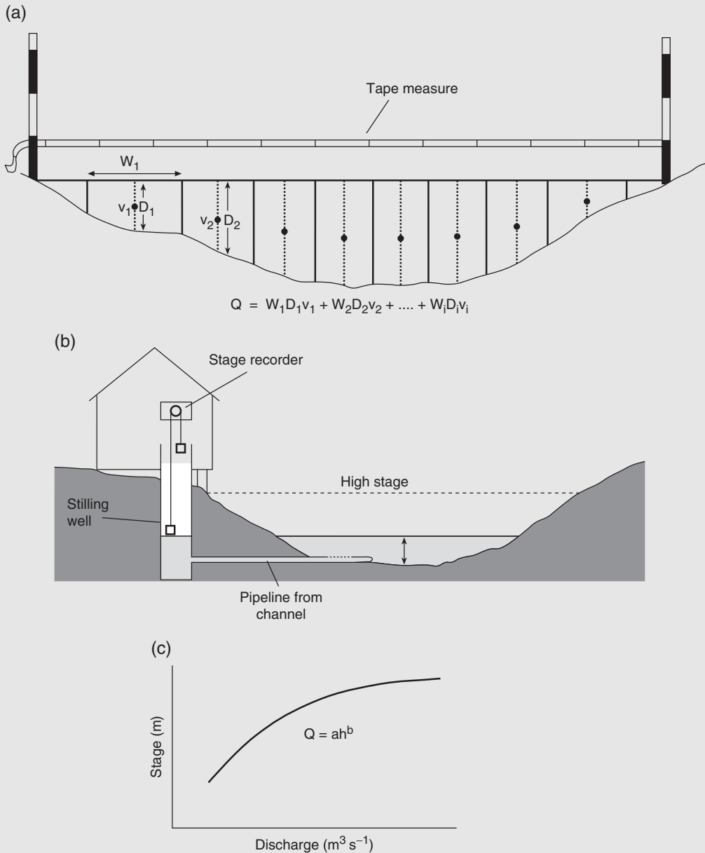
Figure 1 (a) Measuring discharge using the velocity-area method. Q = discharge, D = depth, w = width and v = velocity. (b) Gauging station at a rated section. (c) Rating curve. Q = discharge, h = stage, a and b are coefficients.
