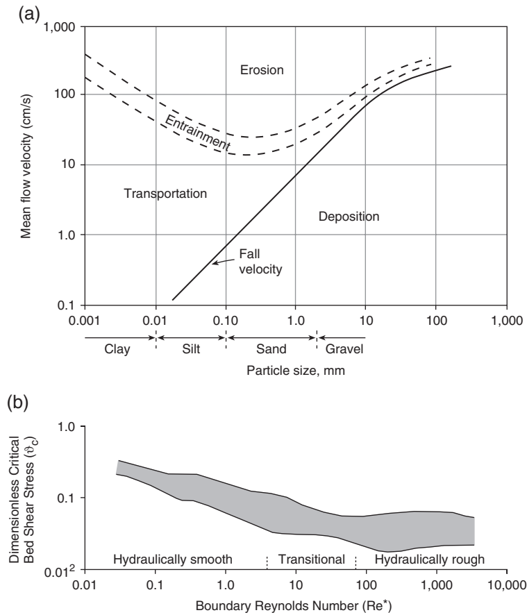
Figure 7.3 (a) The Hjulstrøm diagram, showing the mean flow velocity at which particles of a given size are entrained, transported and deposited. These curves are based on experimental data carried out for well sorted sediments of a uniform size. Adapted from Hjulstrøm (1935). (b) A Shields diagram showing the relationship between the critical dimensionless bed shear stress and the boundary Reynolds number. A large amount of scatter is associated with different experimental conditions and the problem of defining exactly when a threshold has been reached. Adapted from Miller et al. (1977) and Summerfield (1991).
