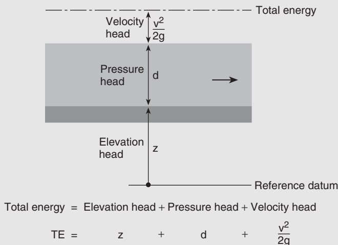
Figure 1 The total energy at a given point in a channel is the sum of the elevation head, pressure head and velocity head at that point. Adapted from Kay (1998).
