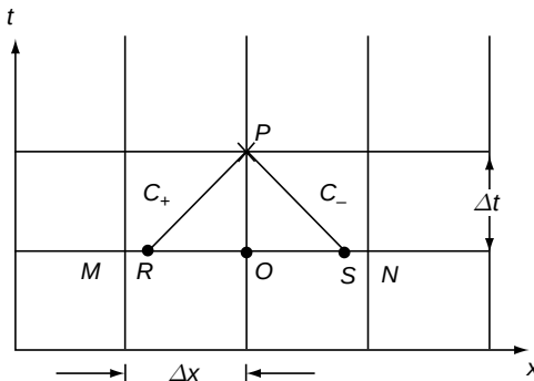
Fig. 10.6 Rectangular grid
