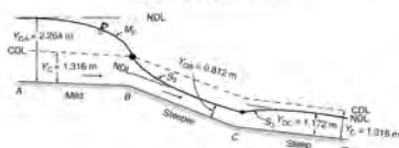
Fig. 4.9 GVF profile for Example 4.1
