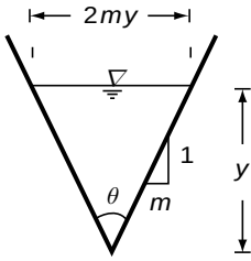
Fig. 2.4 Triangular channel
