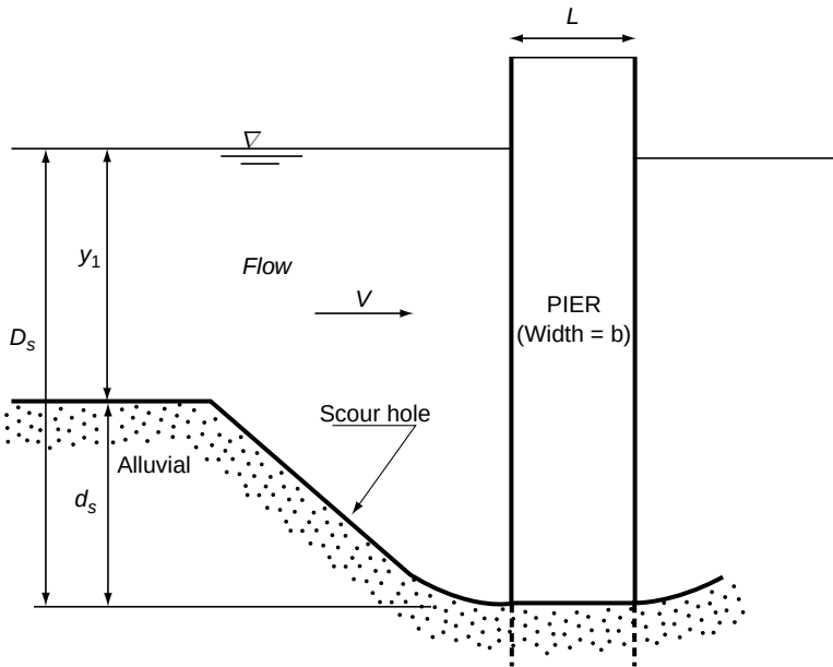
Fig. 11.11 (a) Definition sketch of a scour hole at a bridge pier
