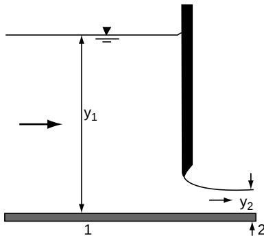
Fig. 1.16 Free flow from a sluice gate – Example 1.8
