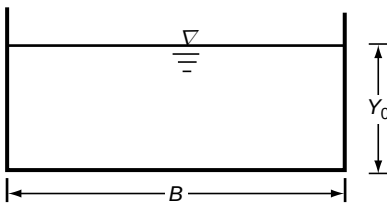
Fig. 3.13 Rectangular channel
