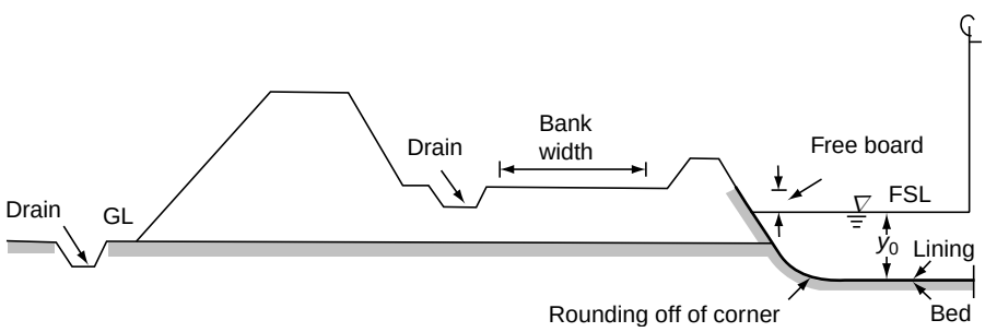
Fig. 3.28 Typical section of a lined irrigation canal
