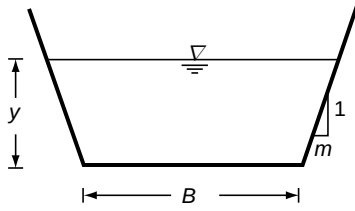
Fig. 2.6 Trapezoidal channel
