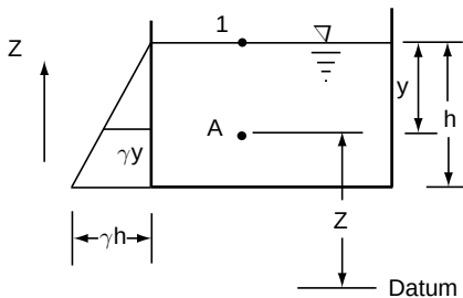
Fig. 1.4(a) Pressure distribution in still water
