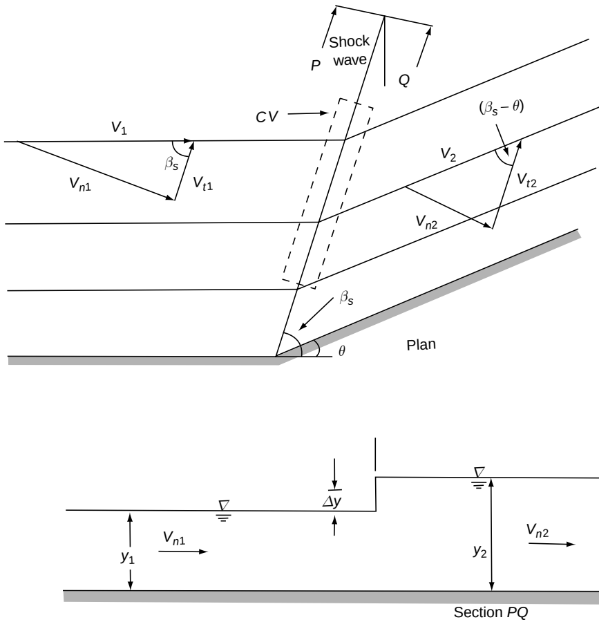
Fig. 9.9 Oblique shock geometry
