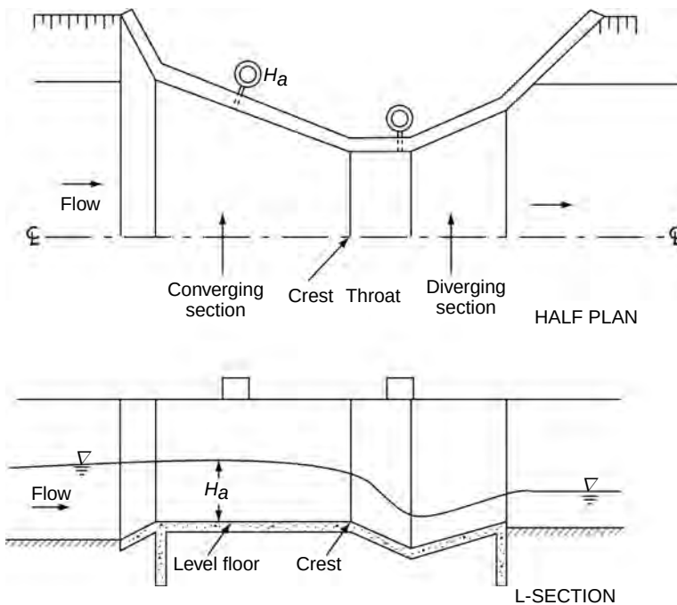
Fig. 7.20 Parshall flume
