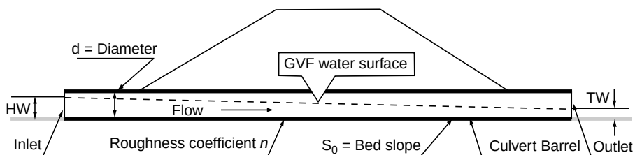
Fig. 7.29 Definition sketch of culvert flow
