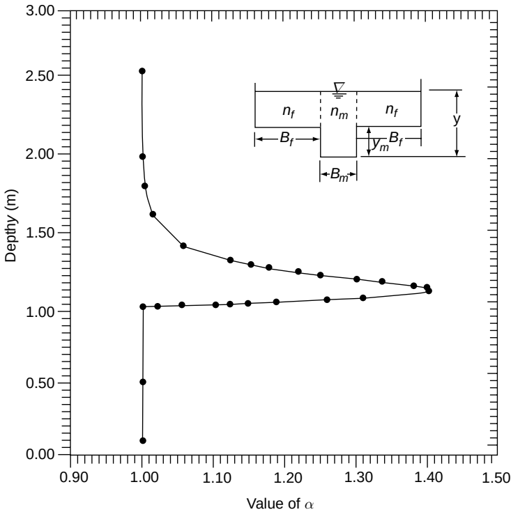
Fig. 5.6 Variation of \alpha with depth in a symmetric compound channel [B_m = 1.0 \text{ m}, B_f = 3.0 \text{ m}, y_m = 1.0 \text{ m}, n_m = 0.013 \text{ and } n_f = 0.0144] .
