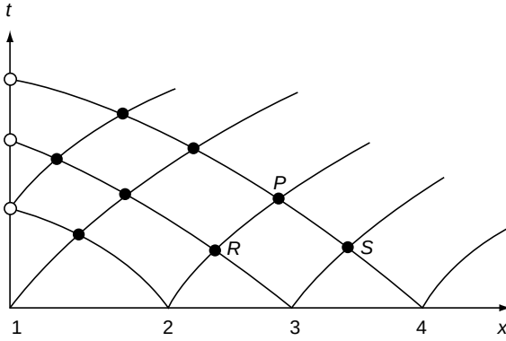
Fig. 10.5 Characteristic grid
