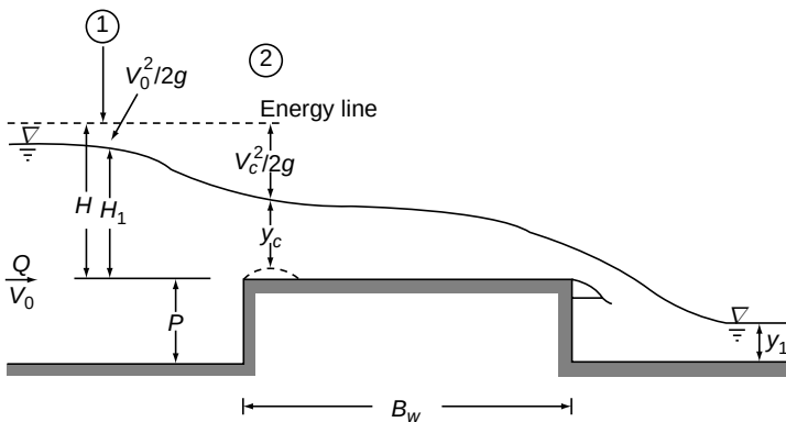
Fig. 7.16 Definition sketch of a broad-crested weir
