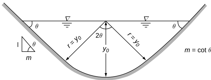
Fig. 3.17 Standard lined triangular channel section for Q \leq 55 \text{ m}^3/\text{s}
