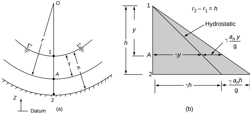
Fig. 1.7 Concave curvilinear flow
