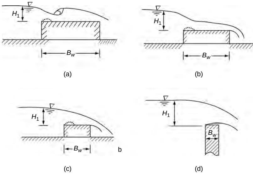
Fig. 7.17 (a) Long-crested weir ( H_1/B_w \lesssim 0.1 ) (b) Broad-crested weir ( 0.1 \lesssim H_1/B_w \lesssim 0.35 ) (c) Narrow-crested weir ( 0.35 \lesssim H_1/B_w \lesssim 1.5 ) (d) Sharp-crested weir ( H_1/B_w \gtrsim 1.5 )
