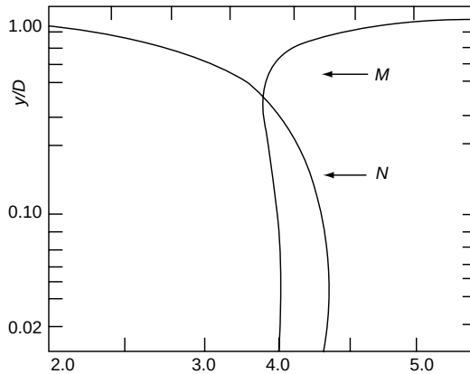
Fig. 5.2 Variation of N and M for a circular channel [6]
