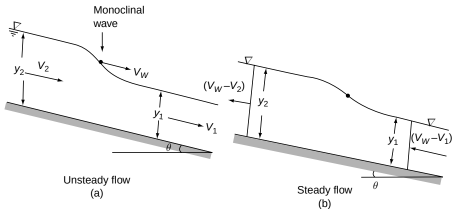
Fig. 10.3 (a) A monoclinical wave (b) Equivalent steady flow
