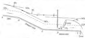
Fig. 4.8 GVF profile for Example 4.1
