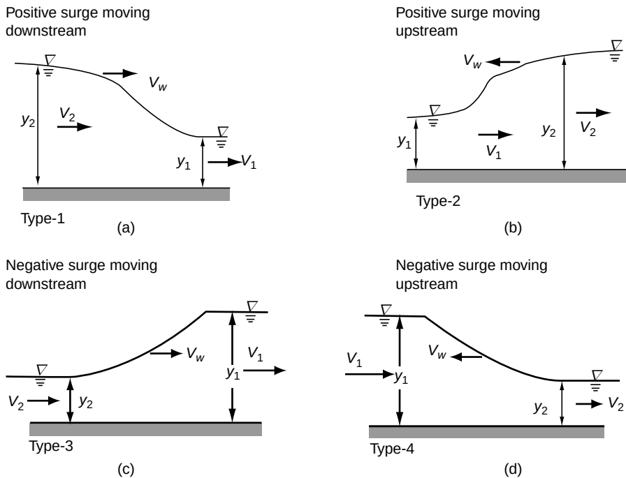
Fig. 10.9 Types of surges
