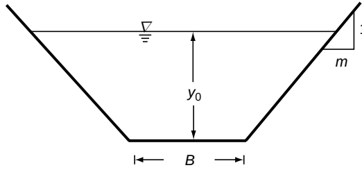
Fig. 3.14 Trapezoidal channel
