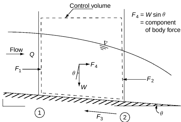
Fig.1.17 Definition sketch for the momentum equation
