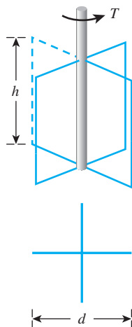
Figure 12.44 Diagram of vane shear test equipment
