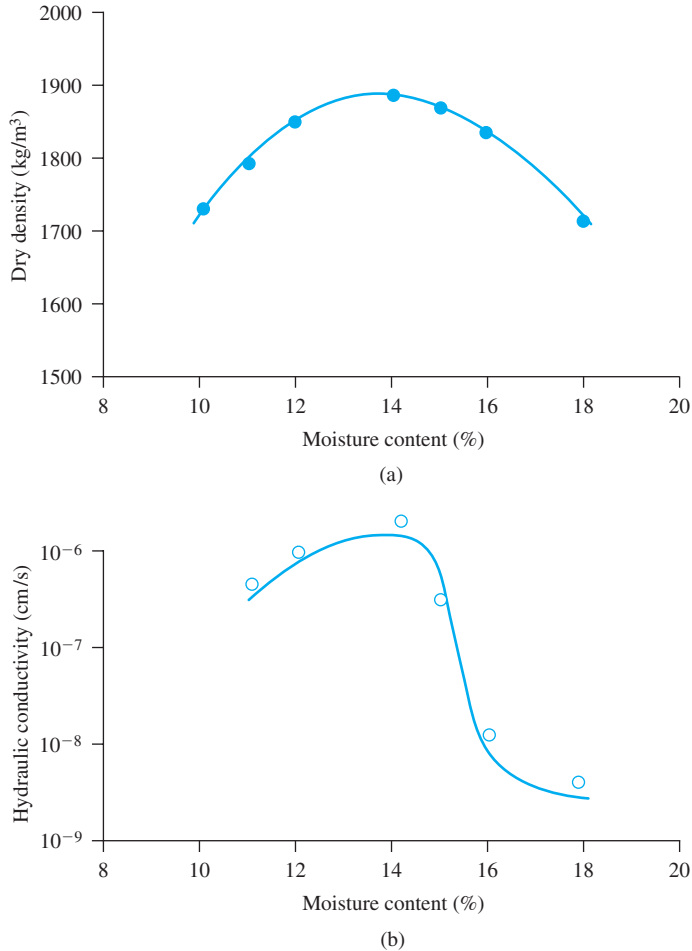
Figure 17.1 Tests on a clay soil: (a) modified Proctor compaction curve; (b) variation of k with molding moisture content
