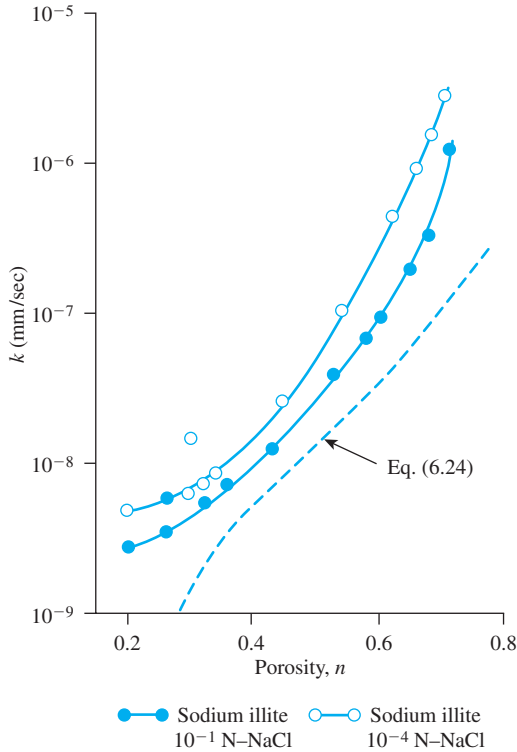
Figure 7.11 Coefficient of permeability for sodium illite (Based on Olsen, 1961)
