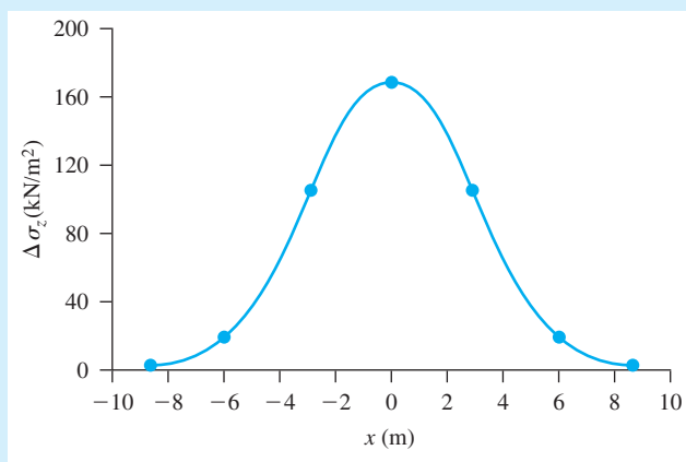
Figure 10.13 Plot of \Delta\sigma_z against distance x
