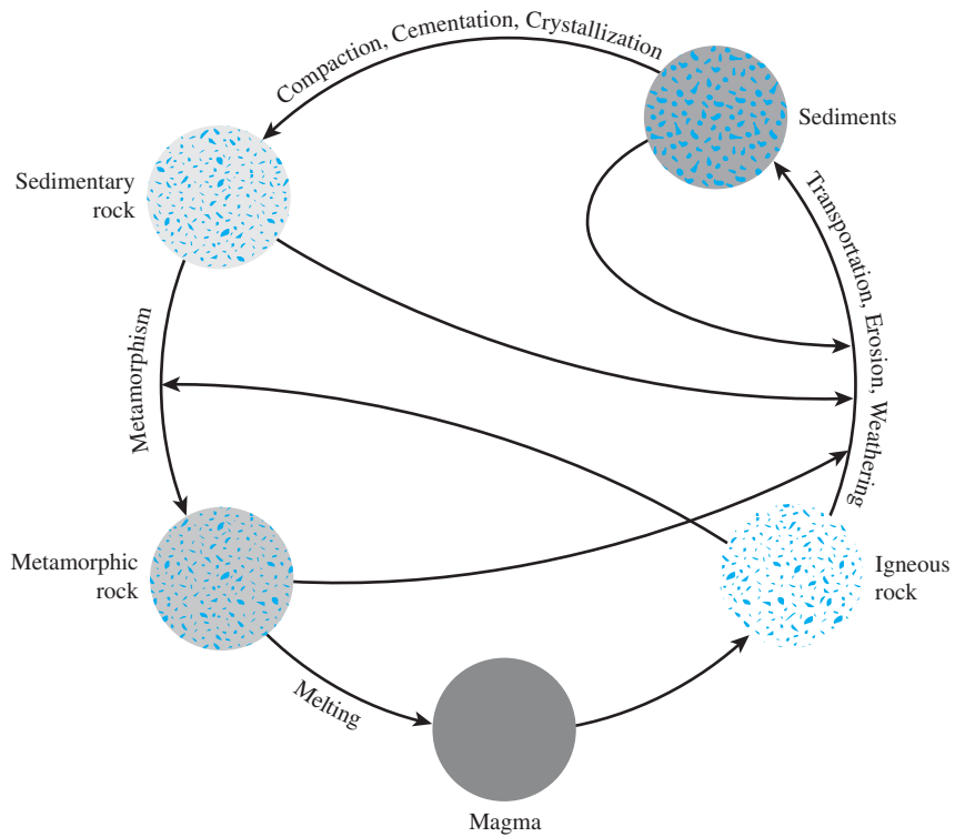
Figure 2.1 Rock cycle
