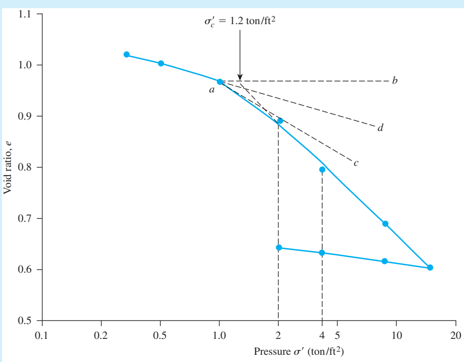
Figure 11.17 Plot of e versus \log \sigma'
