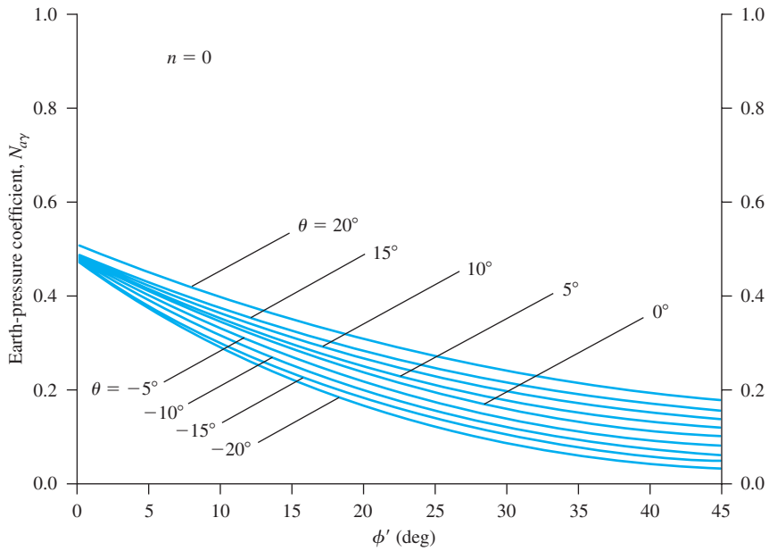
Figure 13.33 Variation of N_{ay} with \phi' and \theta ( n = 0 ) (Based on Prakash and Saran, 1966, and Saran and Prakash, 1968)
