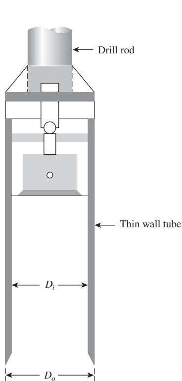
Figure 18.8 Thin-wall tube sampler
