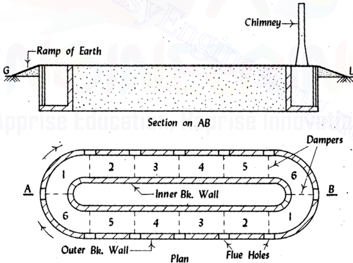
Fig 2.5 Bull's trench kiln
