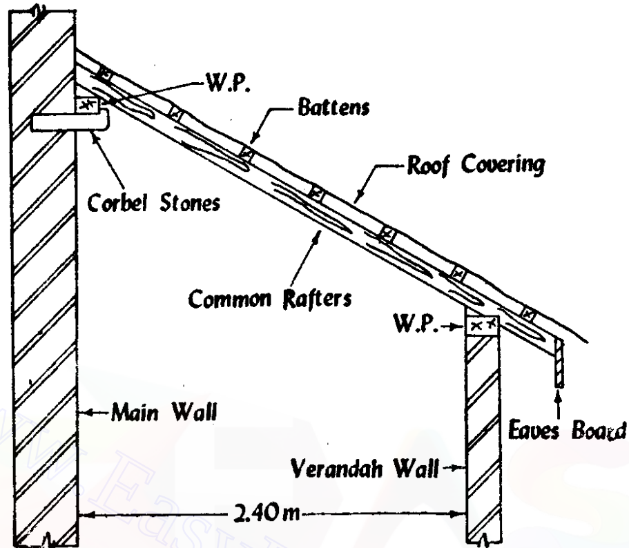
Fig 13.3 Lean-to roof
