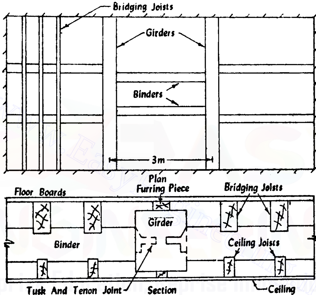
Fig 12.5 Details of framed timber floors
