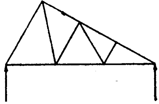
North-light truss
