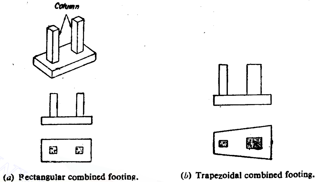
Fig 10.5 Combined Footings
