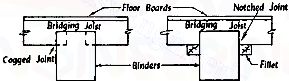
Methods of fixing binders with joists
