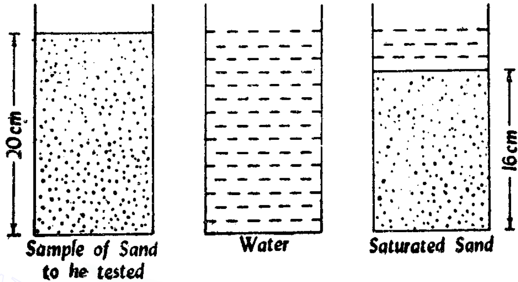
Fig 4.1. Bulking of Sand
