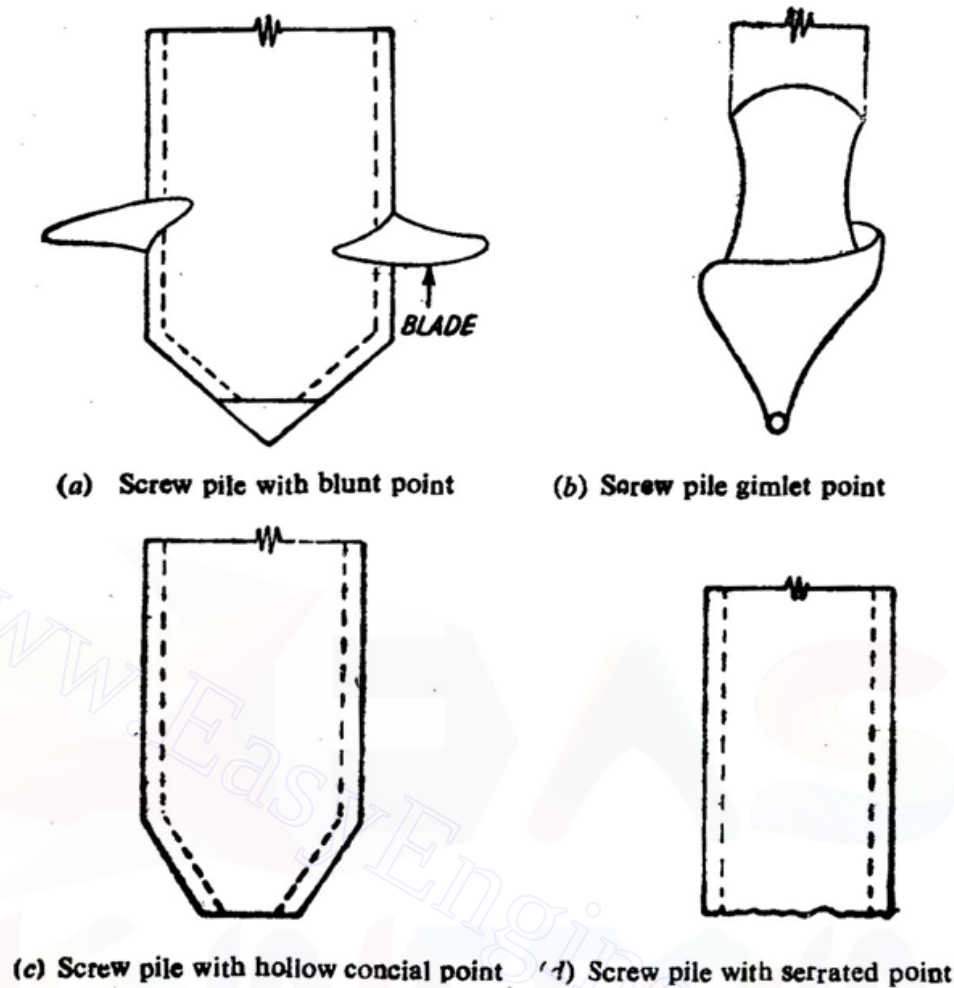
Fig 10.12 Different types of screw piles
