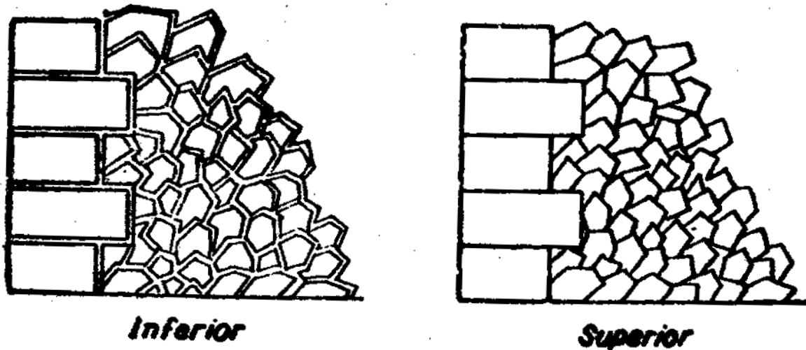
Fig. 11.8 Polygonal rubble masonry
