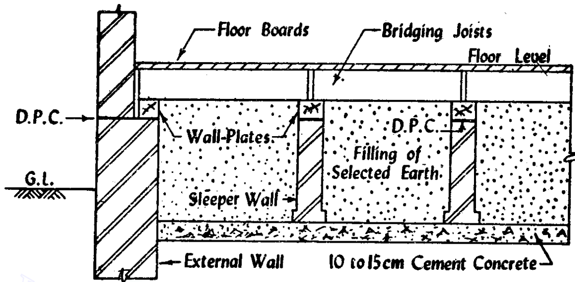
Fig 12.2. Basement or ground floor of timber
