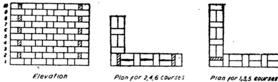
One-brick wall double flemish bond.
