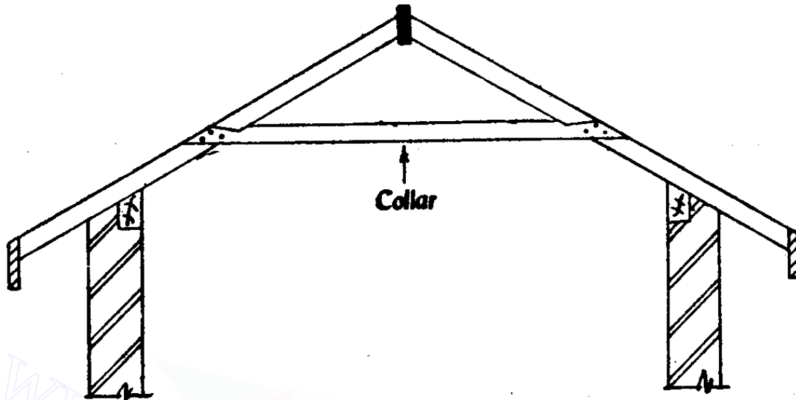
Fig 13.6 Collar beam roof
