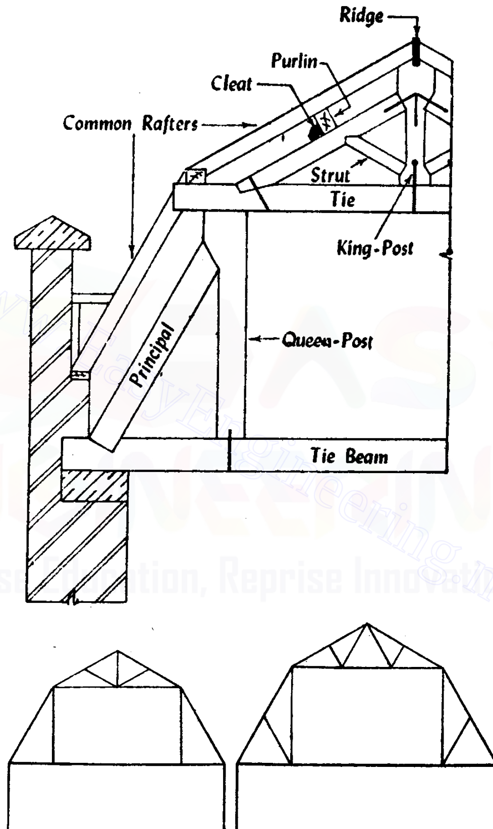
Fig 13.10 Mansard truss
