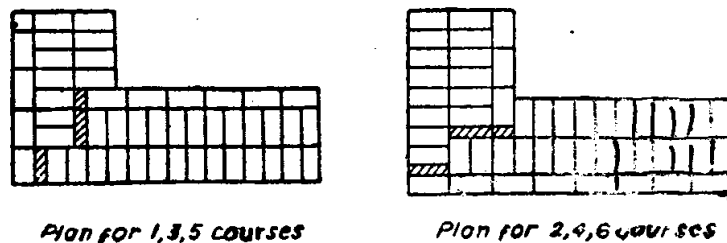
Two-and-a-half-bricks wall English bond.
