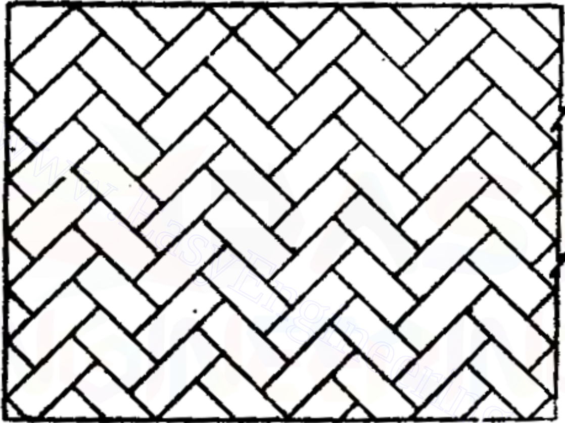
Fig 11.23 Herring Bone Bond
