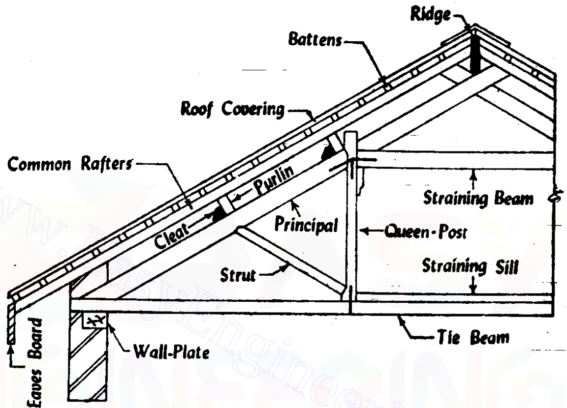
fig 13.9 Queen post truss
