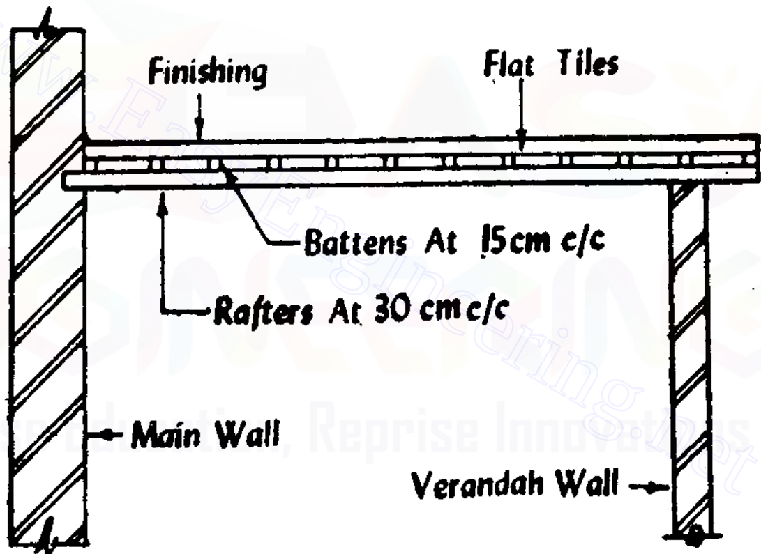
Fig 13.15 Bengal Terrace roof
