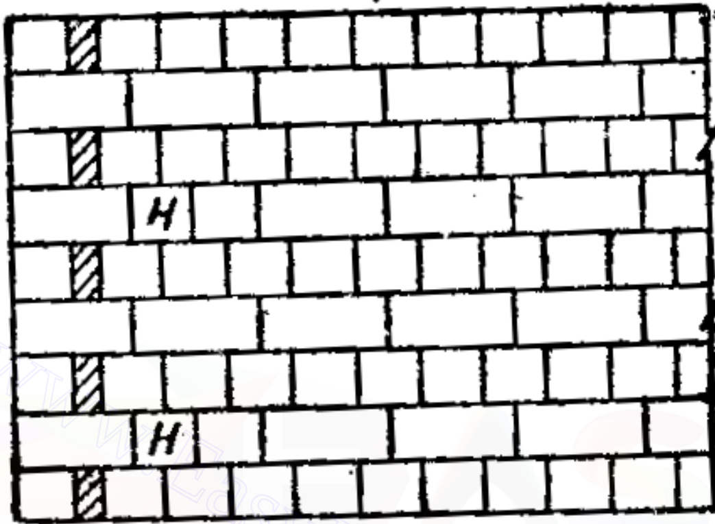
Fig 11.25 English Cross Bond
