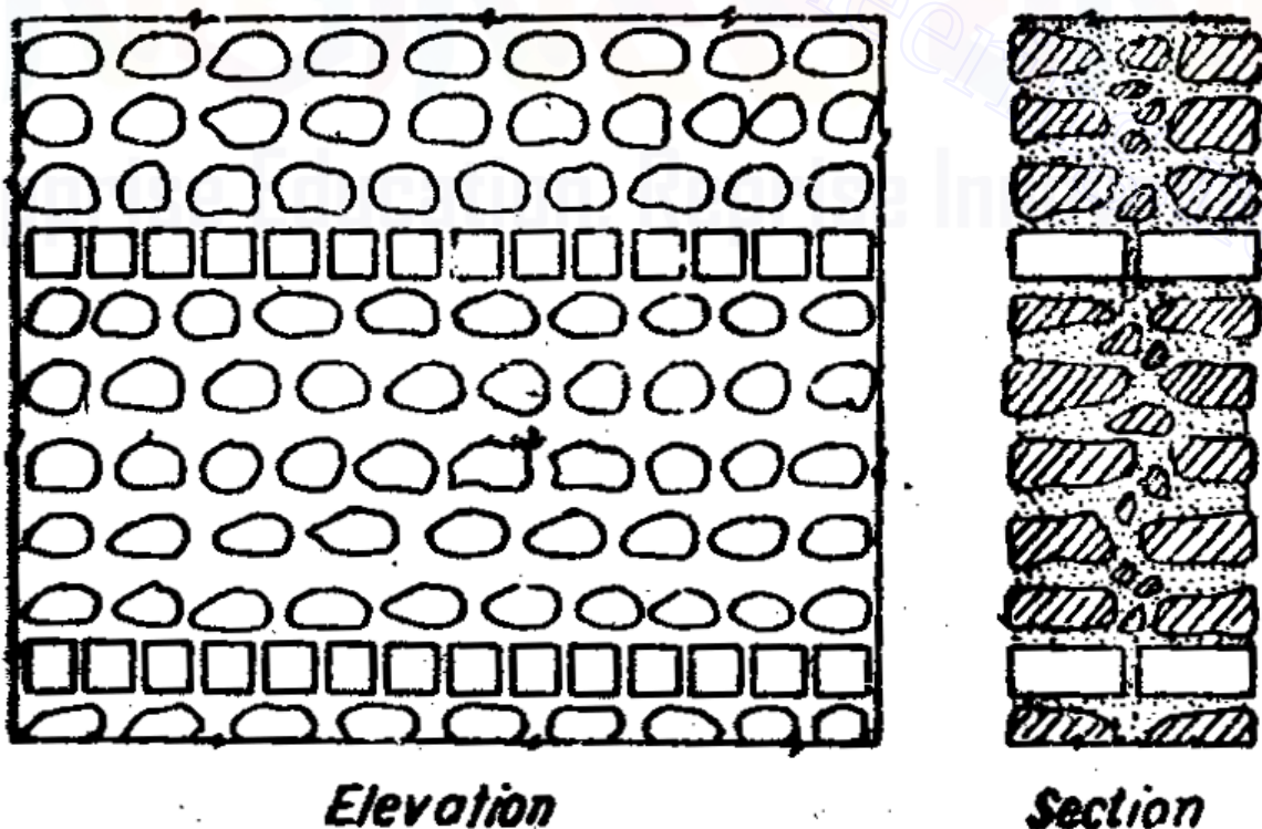
Fig 11.9 Plint Rubble Masonry
