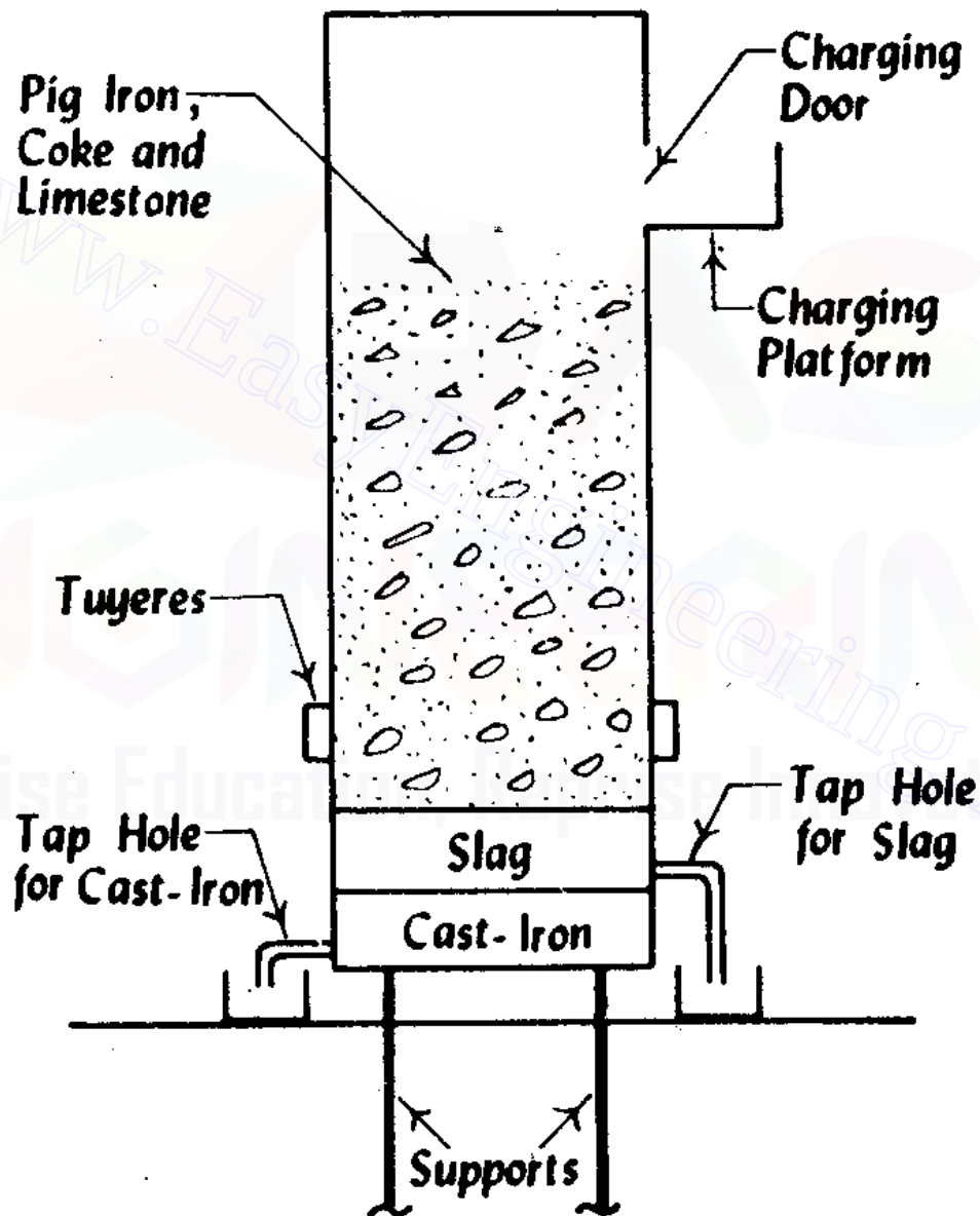
Fig 8.2 Cupola Furnace
