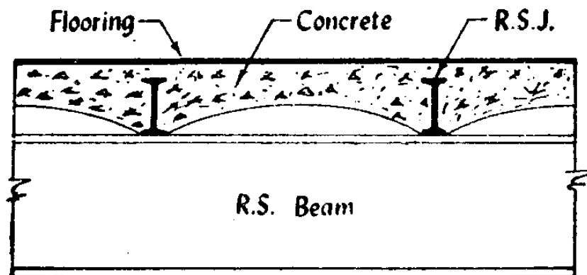
Fig 12.8 (b) Concrete jack floor
