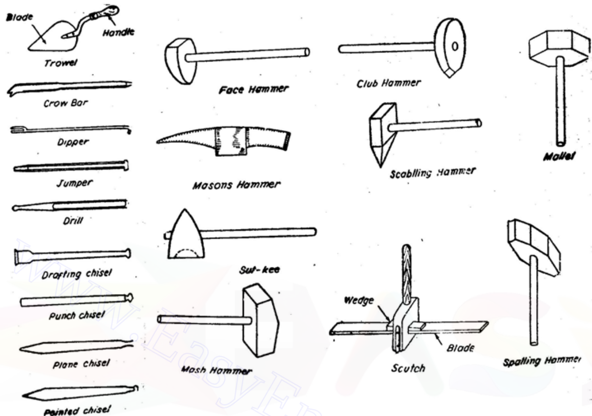
Fig 11.2 Tools for Stone Masonry
