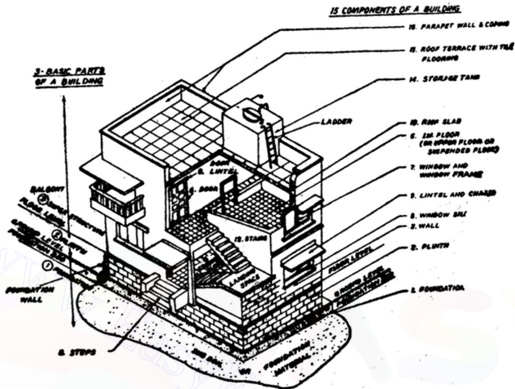
Fig 9.1 Component parts of building
