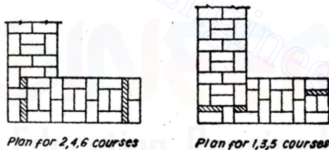
Two-bricks double flemish bond.
