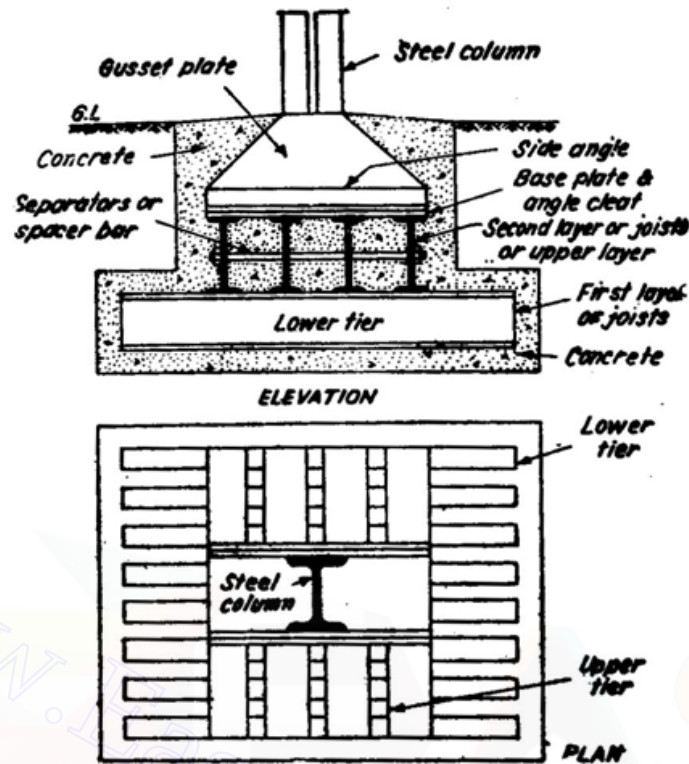
Fig 10.9 Grillage Footing
