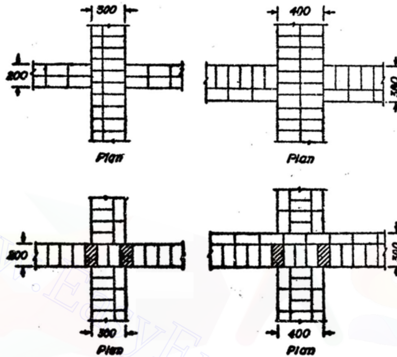
Fig 11.29 Cross Junctions in english bond
