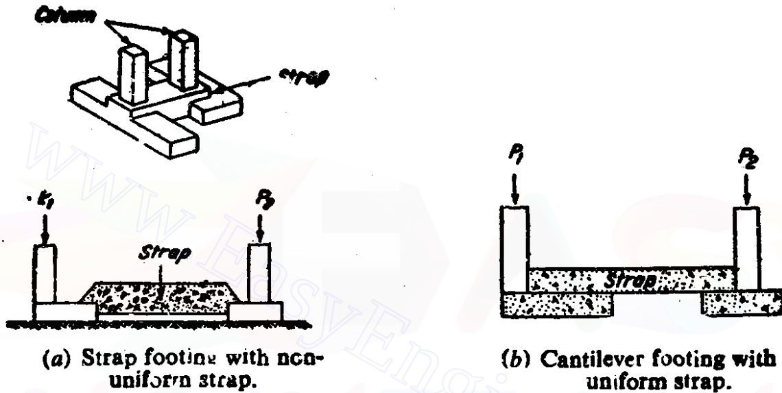
Fig 10.8 Strap or cantilever footing
