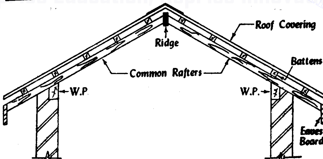
Fig 13.4 Couple roof
