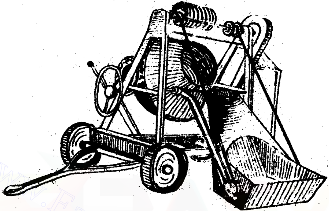
Fig 6.1 Batch type Concrete Mixer
