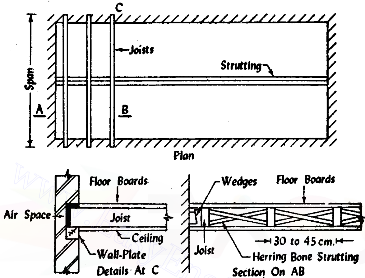
Fig 12.3 Details of single joist timber floor
