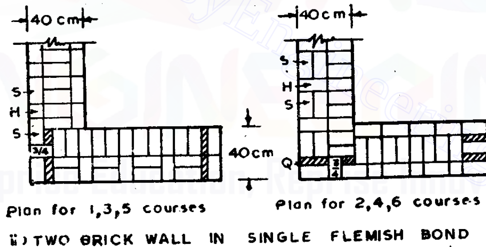
Fig 11.19 Single Flemish Bond
