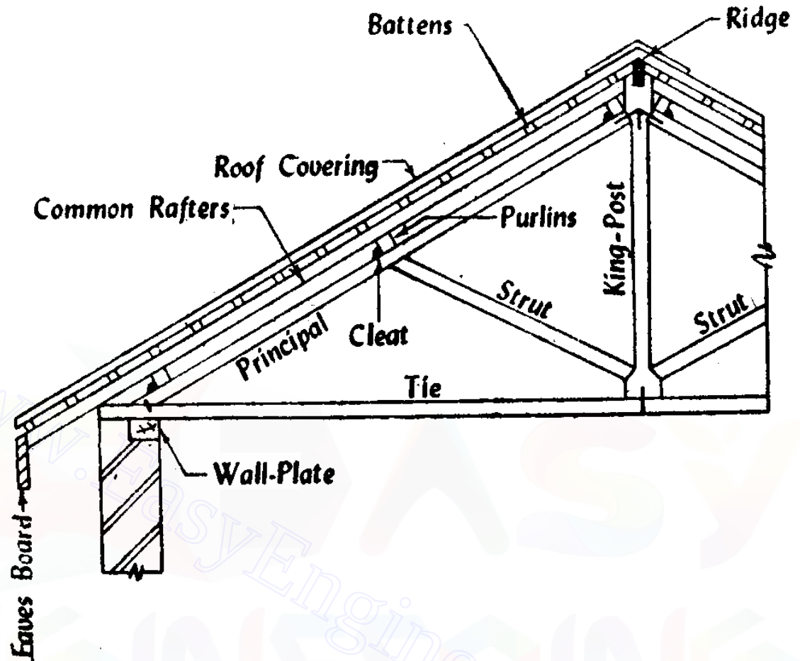
Fig 13.8 King post truss roof
