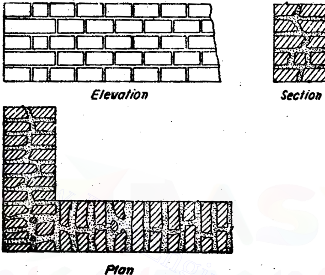
Fig 11.7 Built to regular courses
