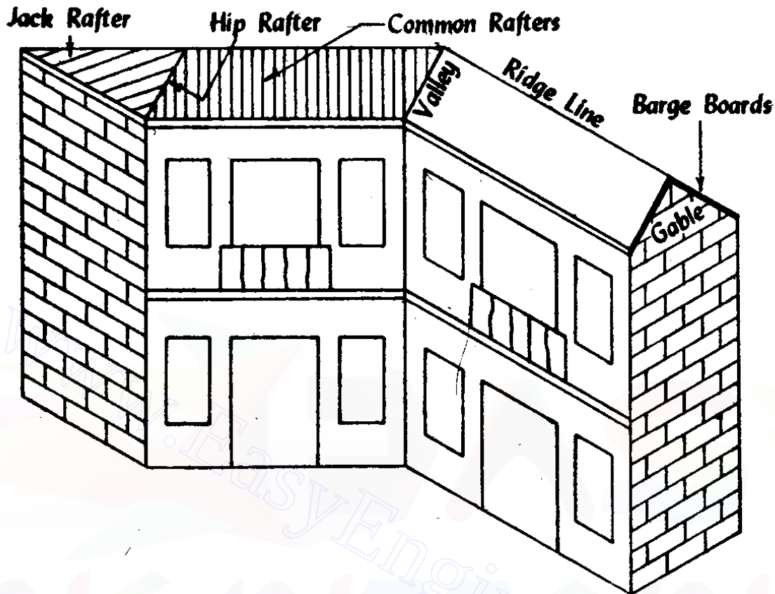
Fig 13.1 Building with pitched roof
