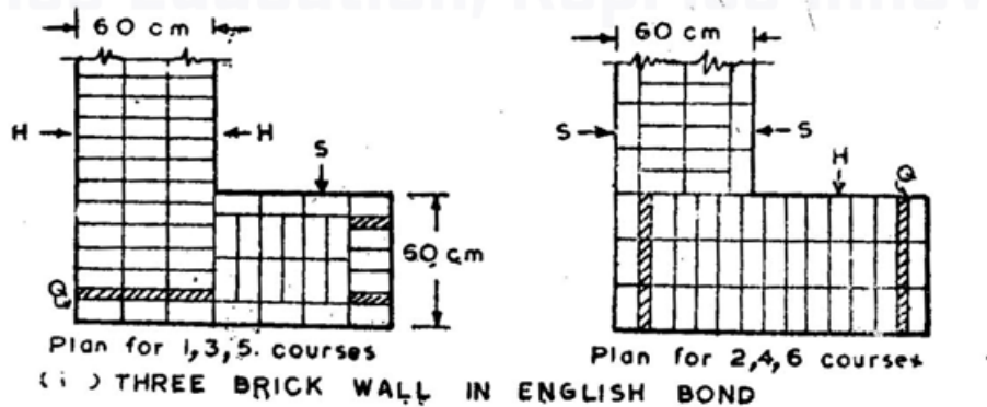
Fig 11.17 Alternate arrangements for various wall thicknesses in English Bond
