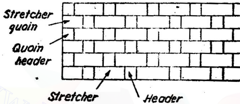
Fig 11.11 Ashlar Fine Masonry
