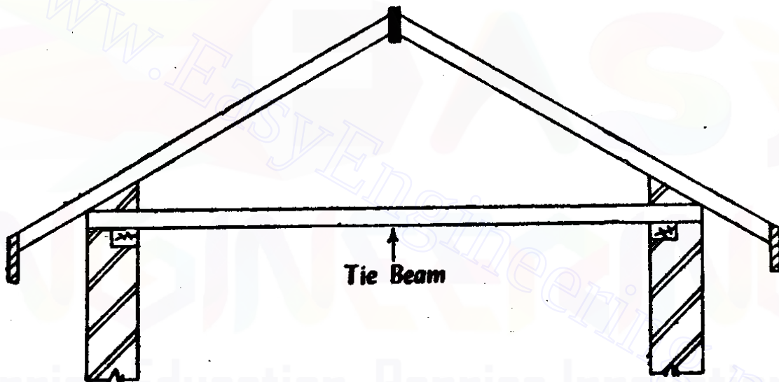
Fig 13.5 Couple close roof
