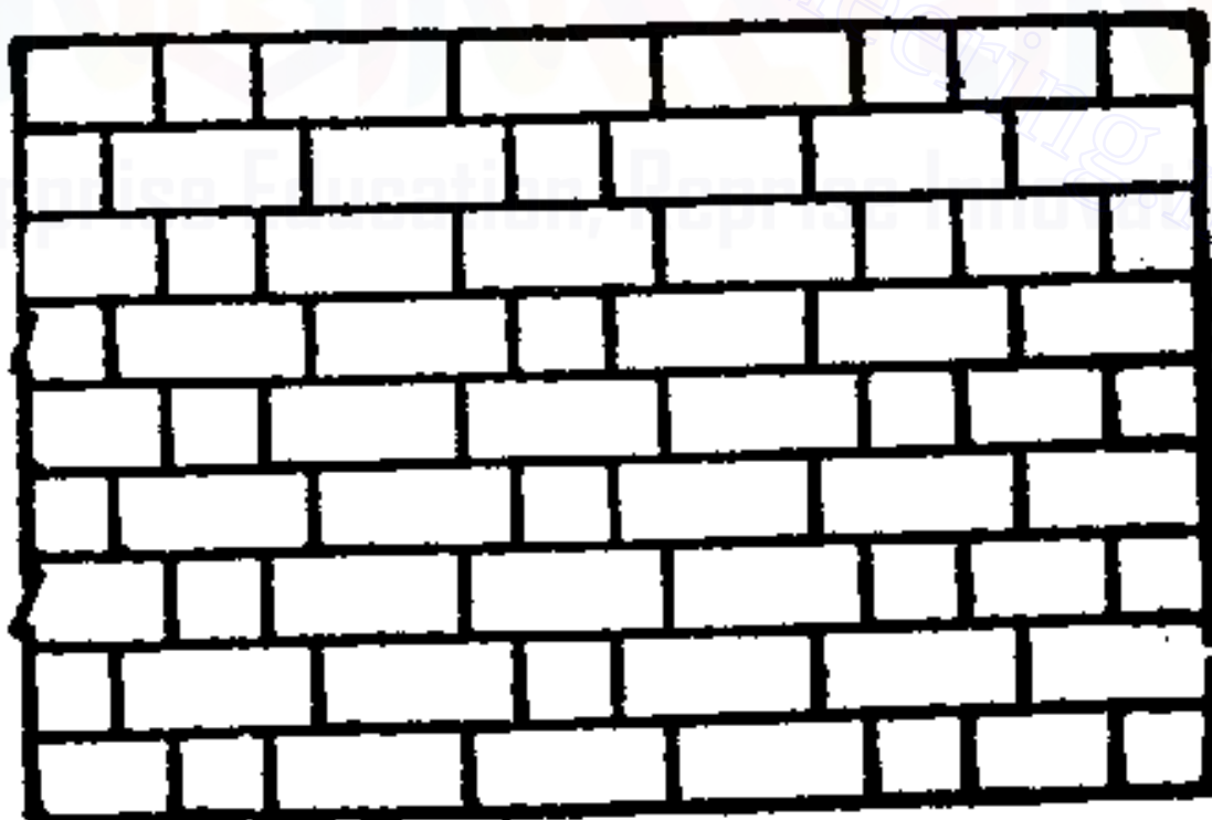
Fig 11.21 Flemish Garden Wall Bond
