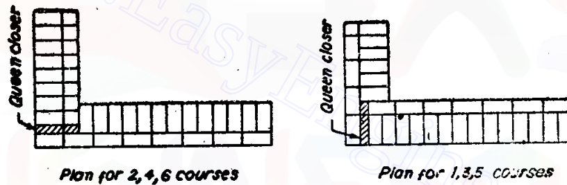
One-and-a-half-bricks wall English bond.
