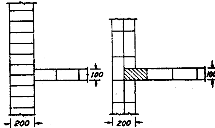
Plans for one-brick Tee-Junction.
