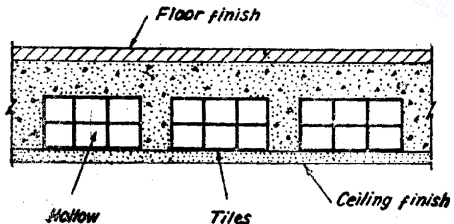
Fire-resisting—Hollow tiled Ribbed floor.
