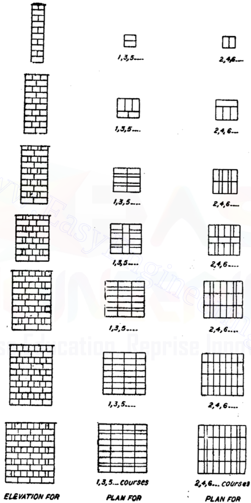
fig 11.26 Bonds in columns
