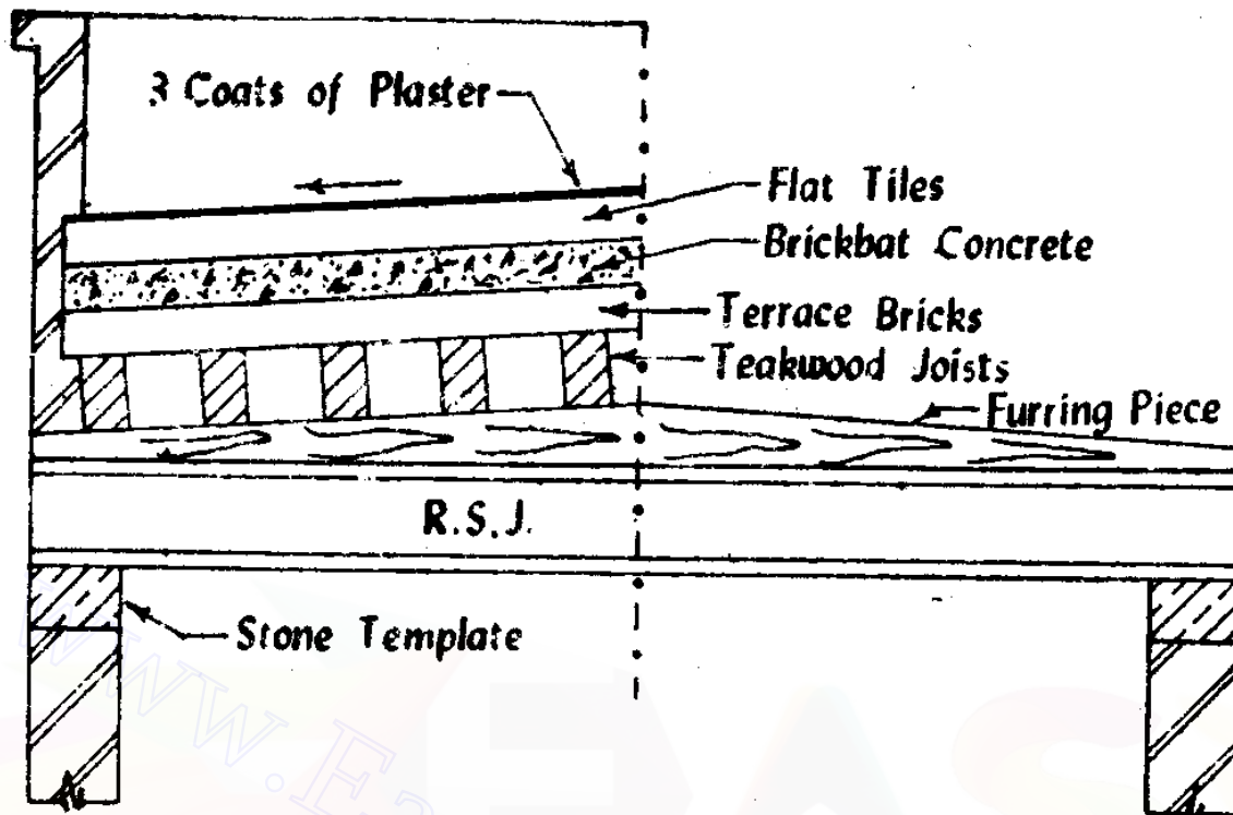
Fig 13.14 Madras Terrace Roof
