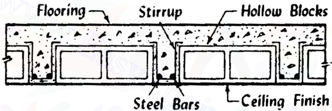
Fig 12.10 Hollow Block and Rib floor
