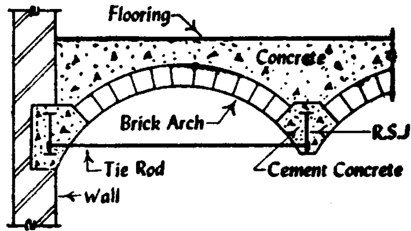
Fig 12.8 (a) Brick Jack arch floor
