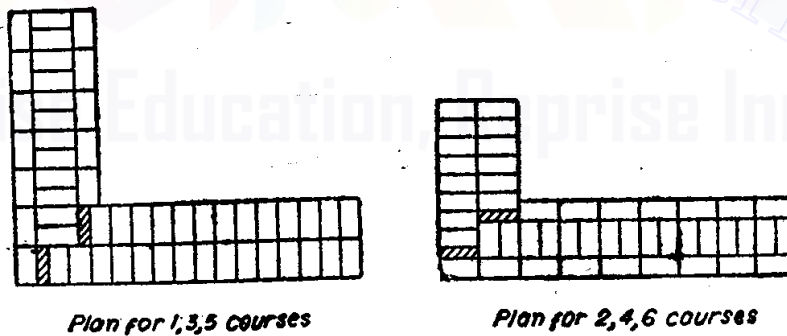
Two-bricks wall English bond.
