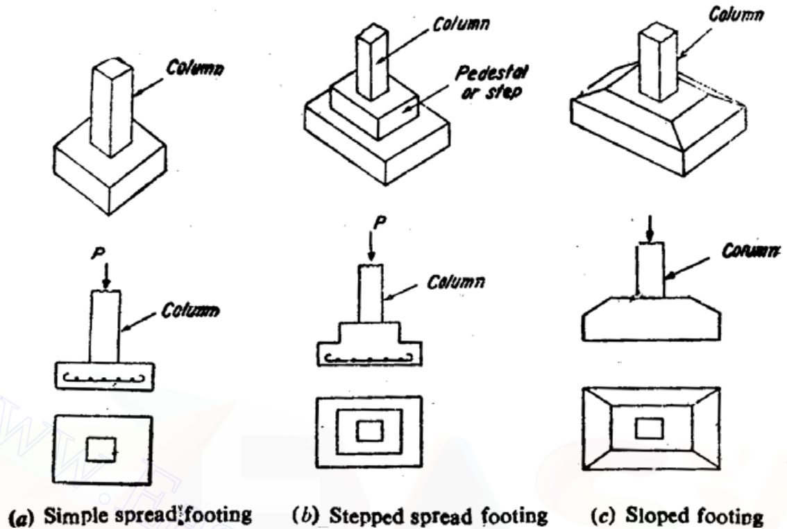
Fig 10.4 Types of Isolated Footings
