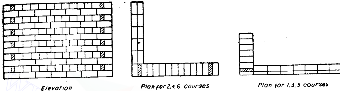
One-brick wall English bond
