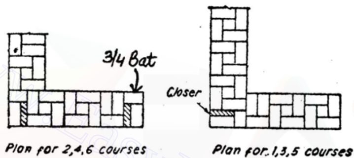
One-and-a-half-bricks double flemish bond.
