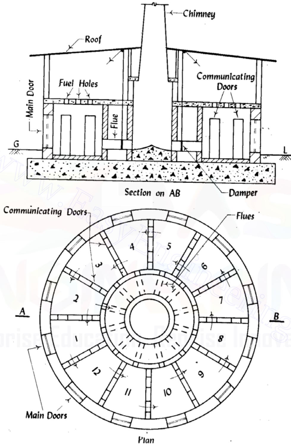
Fig 2.6 Hoffman's kiln
