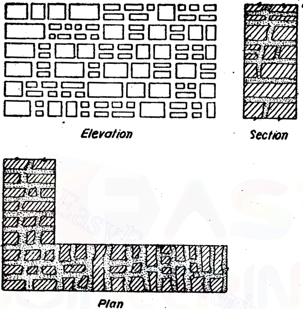
Fig 11.6 Coursed Squared Rubble Masonry
