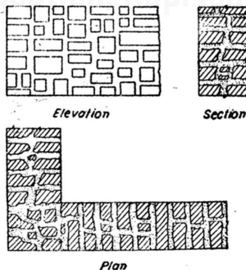
Fig 11.4 Uncoursed squared rubble masonry
