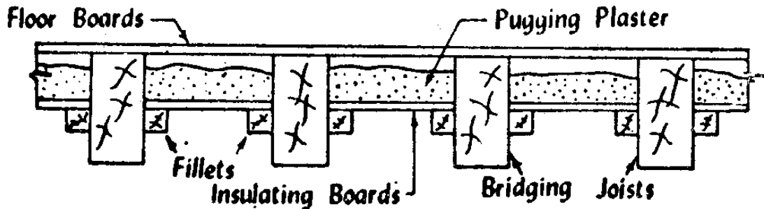
Fig 12.1 Pugging
