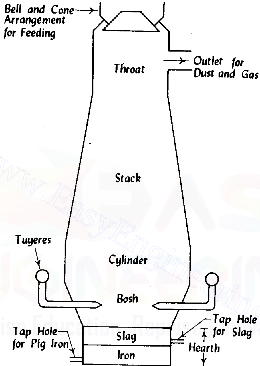
Fig 8.1 Blast Furnace
