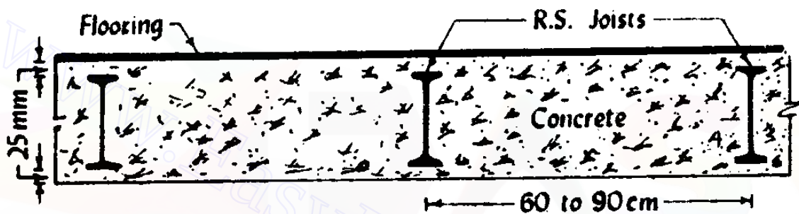
Fig 12.7 Filler Joist Floor
