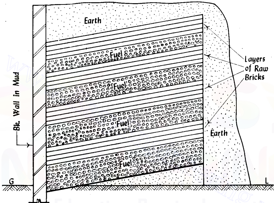
Fig 2.3 Clamp
