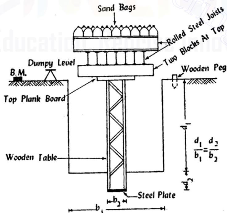
Fig 10.1 Method of loading
