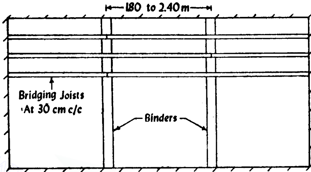
Plan of double joist timber floor
