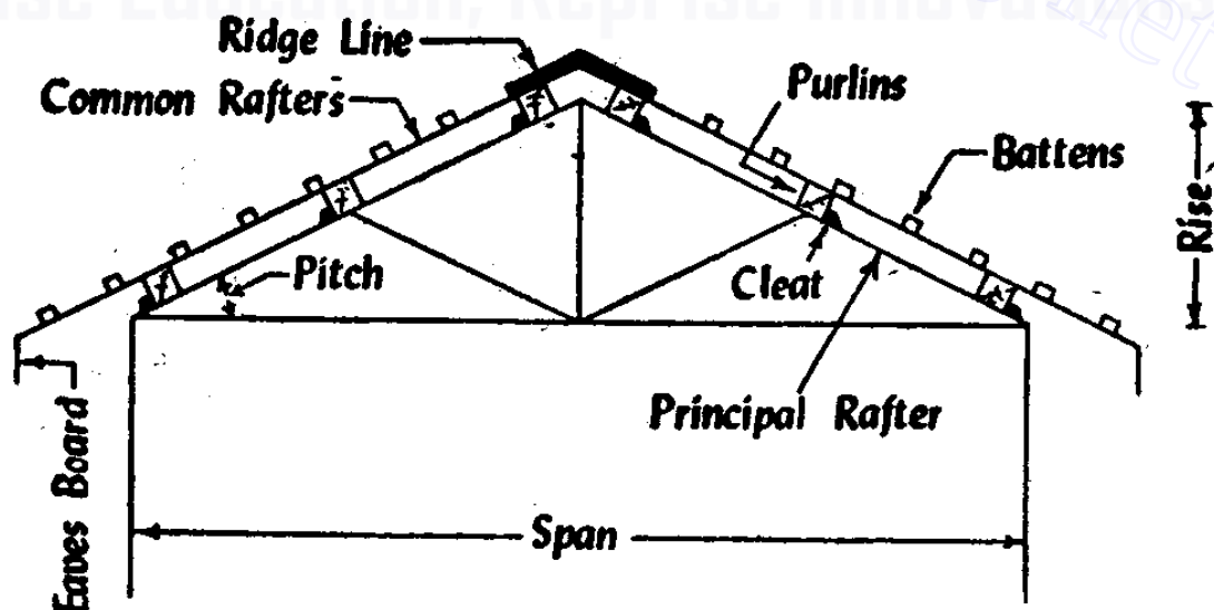
Fig 13.2 Truss
