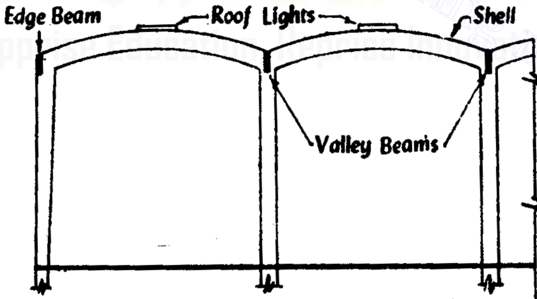
Fig 13.17 Barrel vault shell roof
