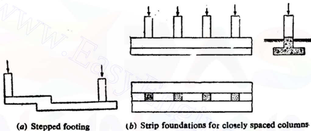
Fig 10.7 Continuous Footing
