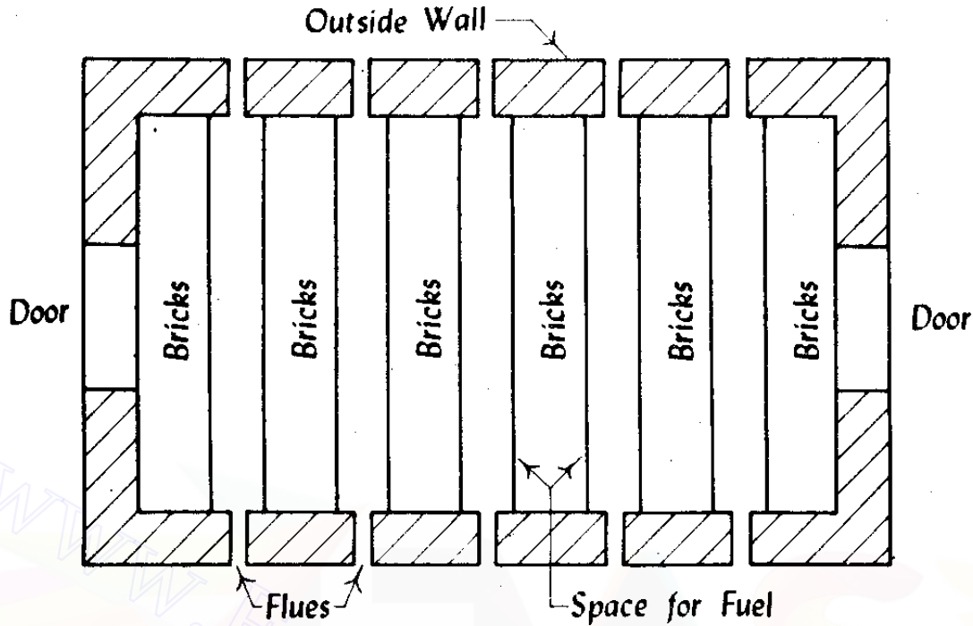
Fig 2.4 Intermittent kiln
