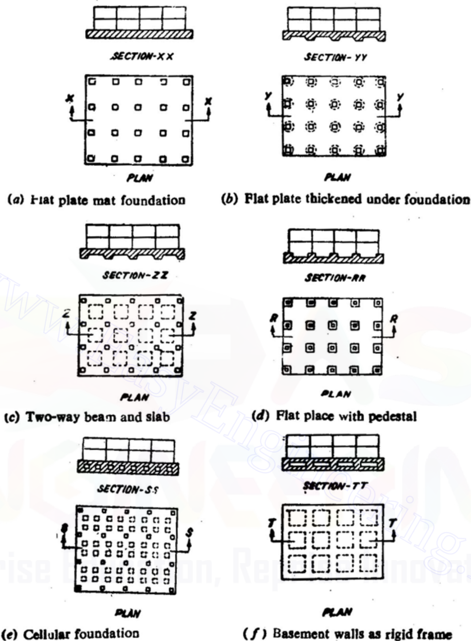
Fig 10.10 Different types of Raft Foundations
