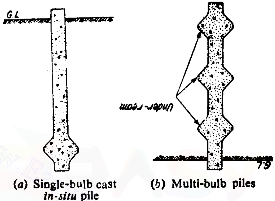
Fig 10.14 Under-reamed Piles
