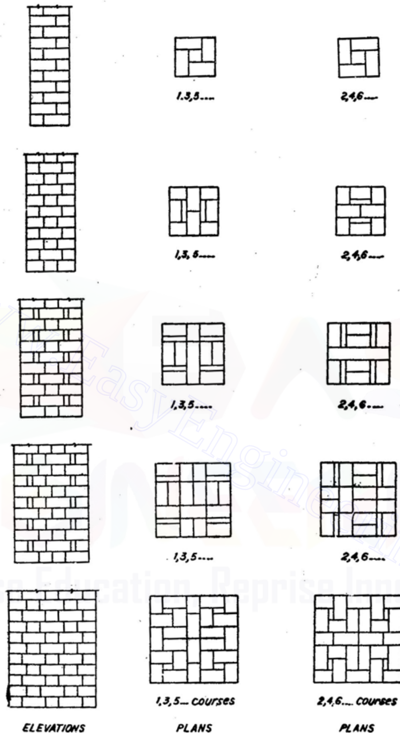
Fig 11.27 Columns in Double Flemish bond
