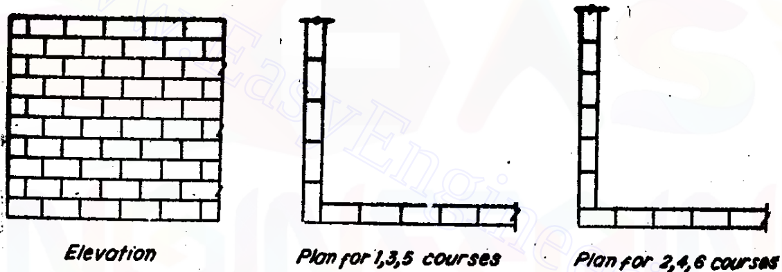
Fig 11.14 Stretcher Bond
