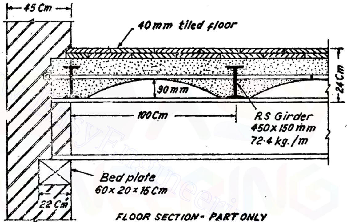
Fire-resisting concrete Jack Arch floor.
