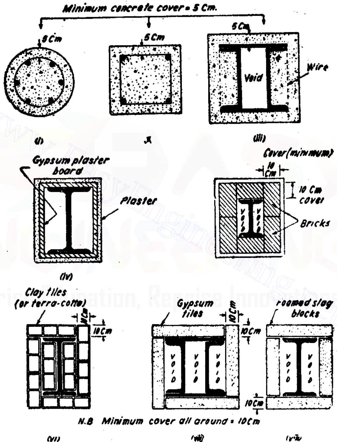
Fig 14.3 Fire proofing treatments to concrete and steel columns
