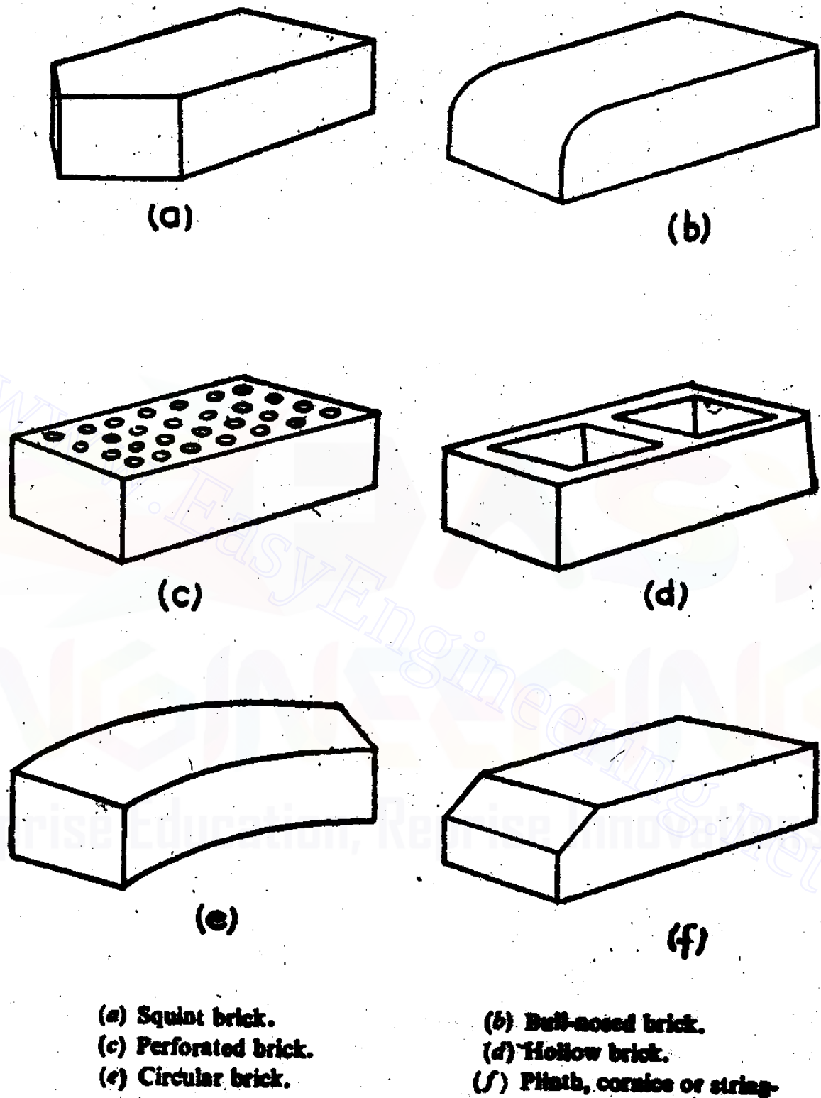
Fig 2.7 Types of Special Bricks
