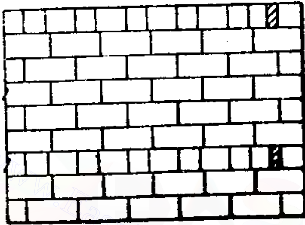
Fig 11.20 English Garden Wall Bond
