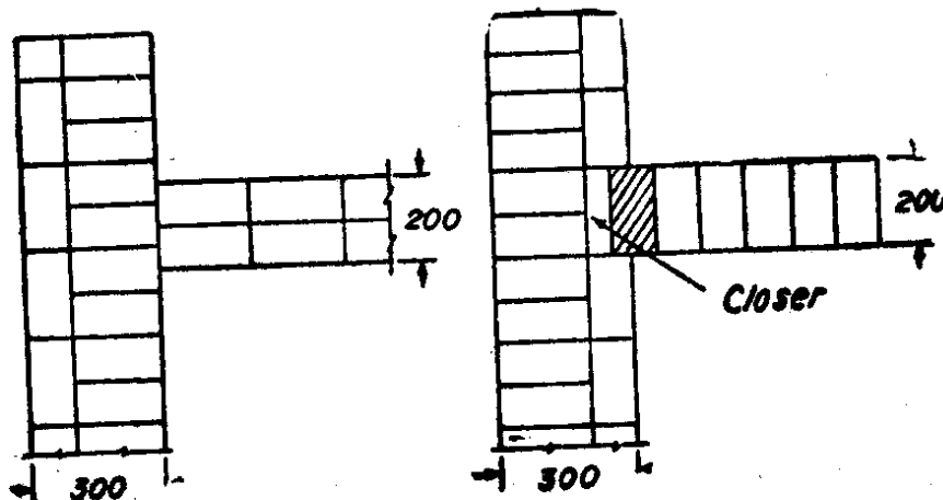
Fig 11.28 Bonds in Tee-Junction
