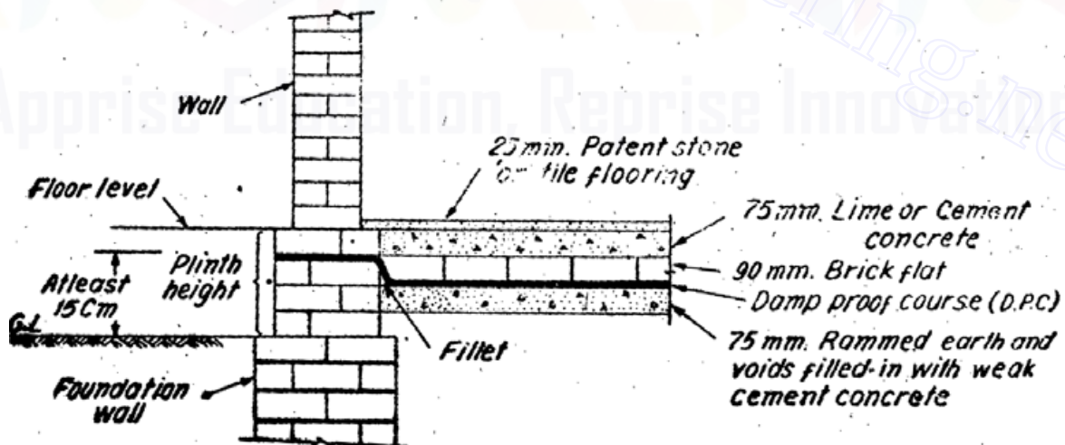
Fig 14.1 D.P.C. above ground level for new buildings
