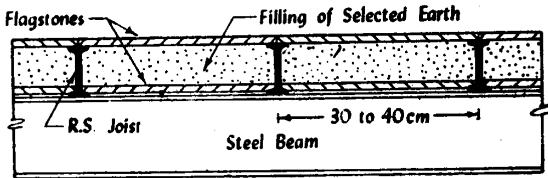
Fig 12.6 Double Flagstone floor
