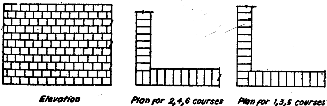
Fig 11.15 Header Bond
