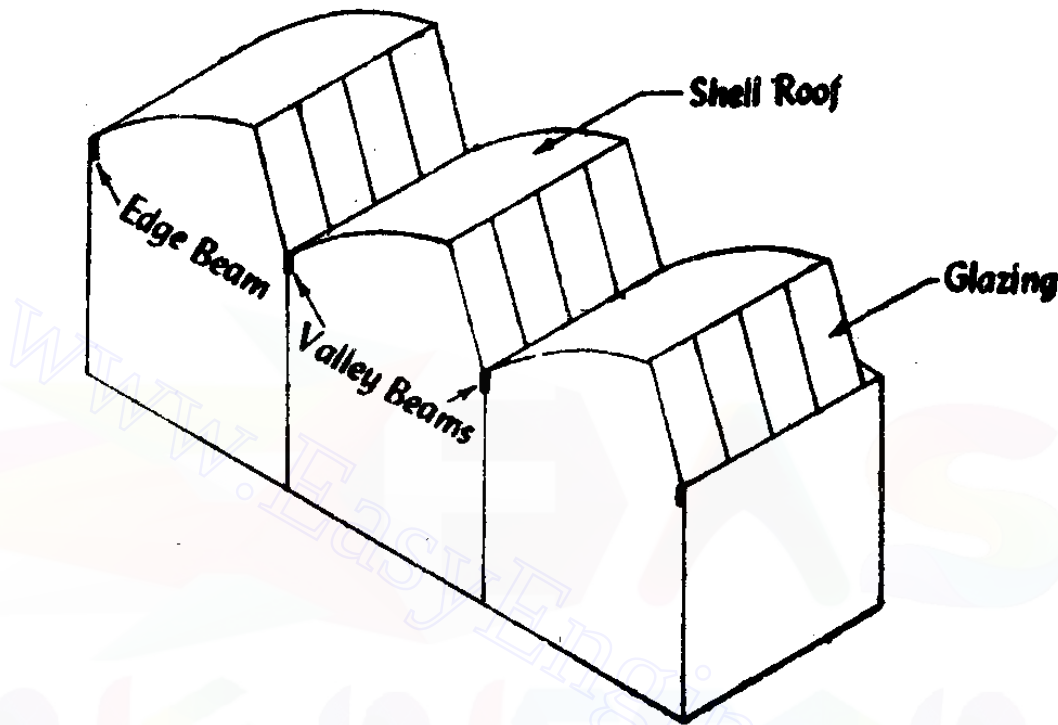
Fig 13.16 North-light shell roof
