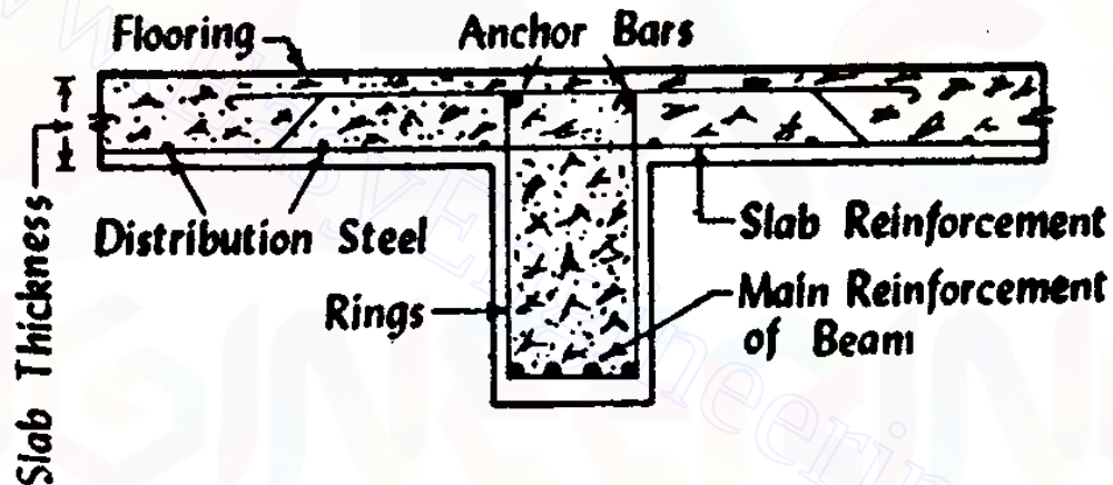
Fig 12.9 R.C.C. Floor
