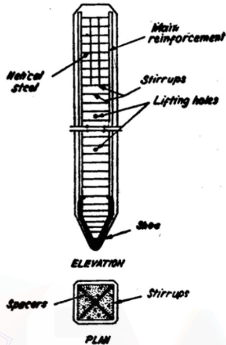
Fig 10.13. Pre-cast concrete Pile
