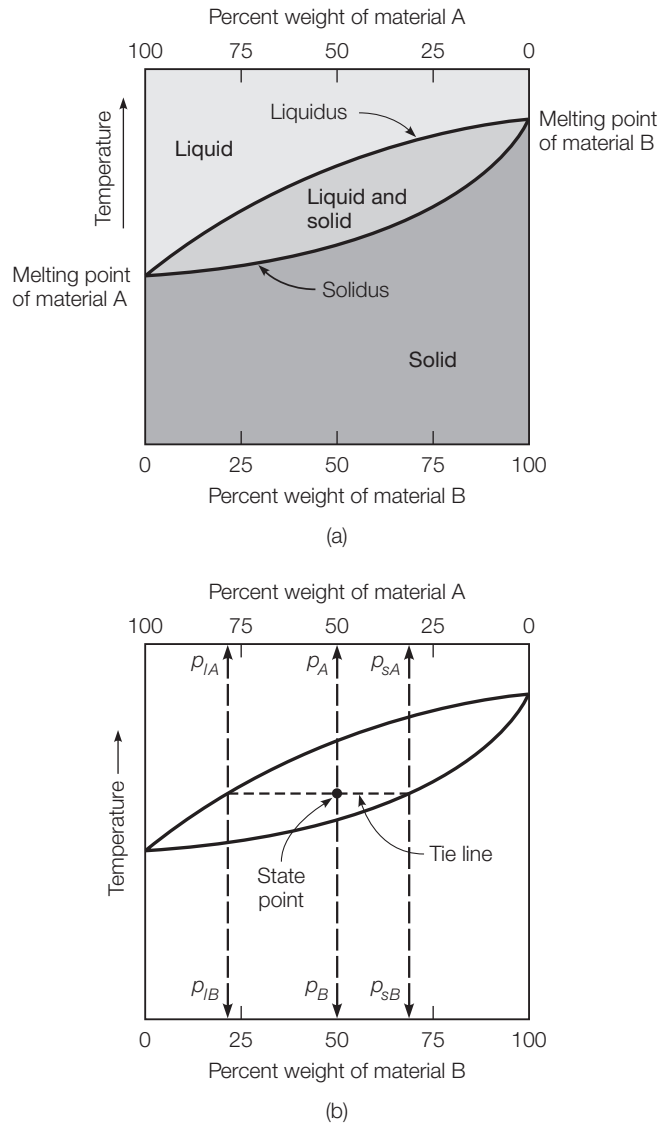
FIGURE 2.14 Binary phase diagram, two soluble elements.
