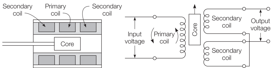
FIGURE 1.28 LVDT circuit.
