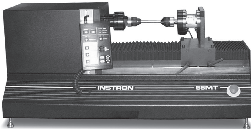
FIGURE 3.20 Torsion test apparatus. (Courtesy of Instron®)
