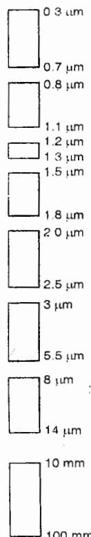
FIG. 16.4 ATMOSPHERIC WINDOWS
