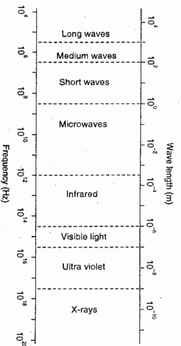
FIG. 15.2 ELECTROMAGNETIC SPECTRUM.
