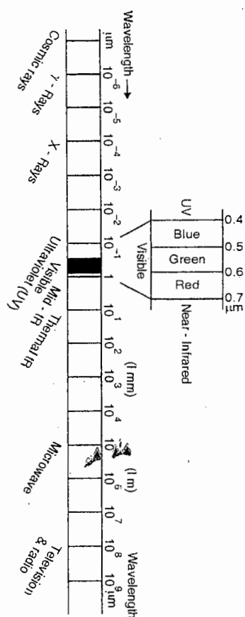
FIG. 16.3. ELECTROMAGNETIC SPECTRUM
