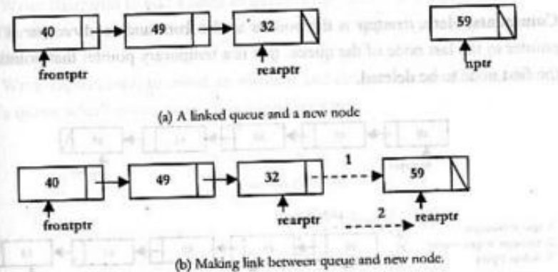
Figure-6.8: Add a new node to a linked queue
