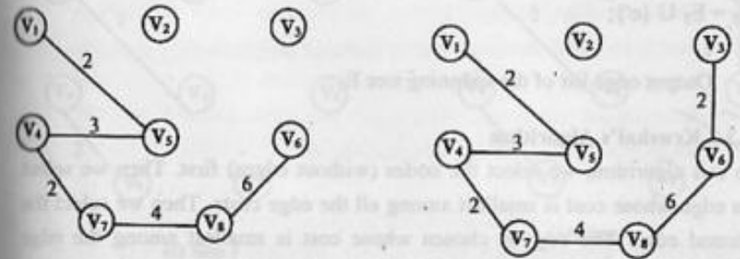
(e) Selection of fifth edge We cannot select the edge (V_8, V_4) , it has been already selected and we reject (V_8, V_5) , since it makes a cycle
