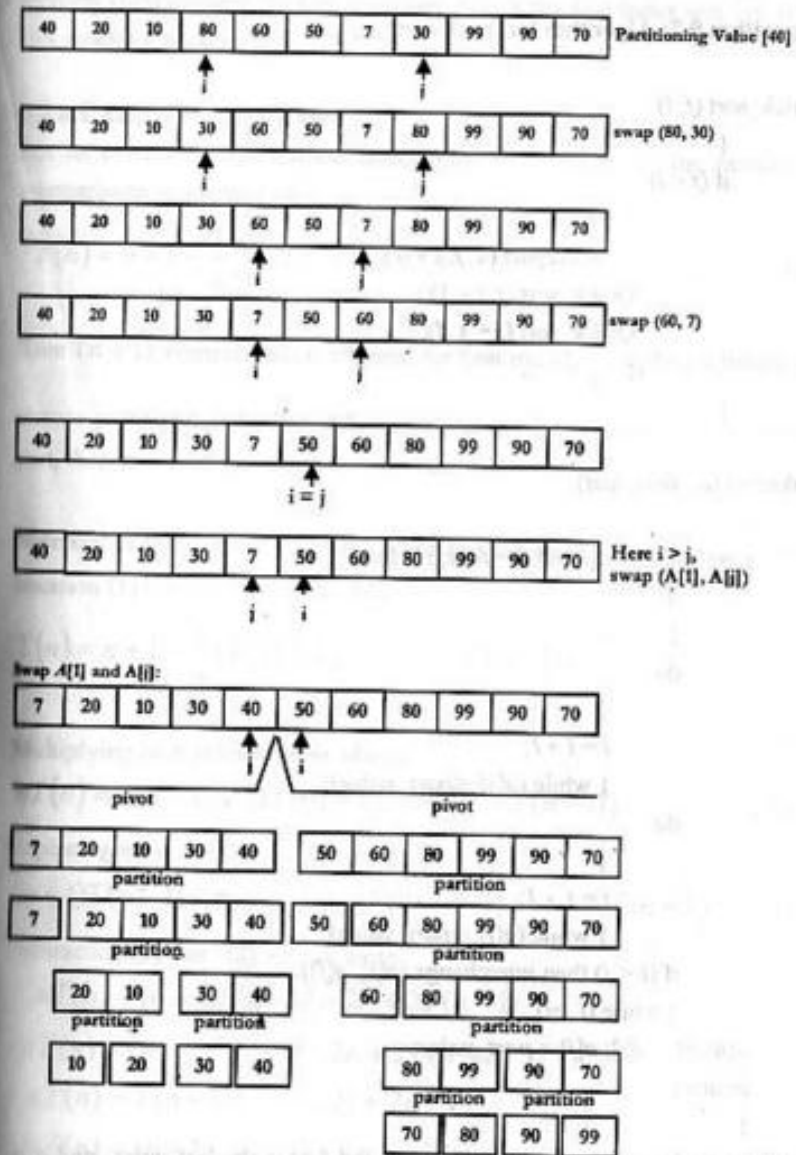
Figure-9.8: Pictorial view of quicksort partitioning
