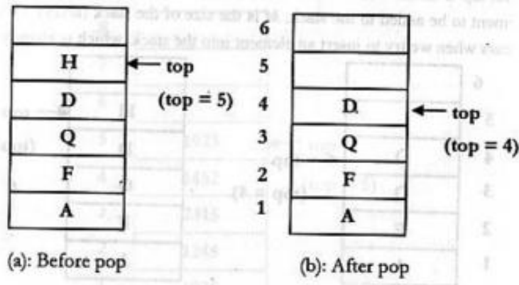
Figure-5.3: Pictorial view of pop operation
