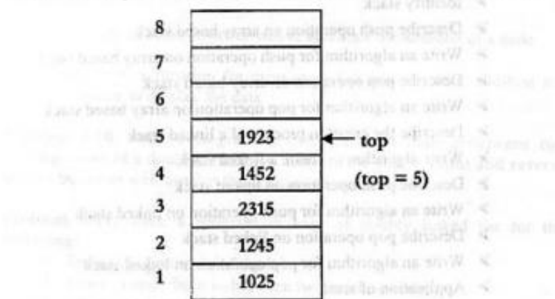
(a) An array based Stack
