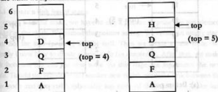
(b): After push
