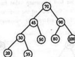
a) A binary search tree
