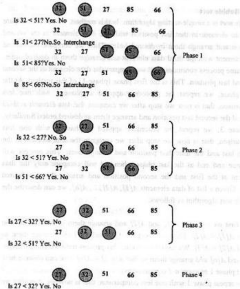
Figure-9.5: Pictorial view of bubble sort
