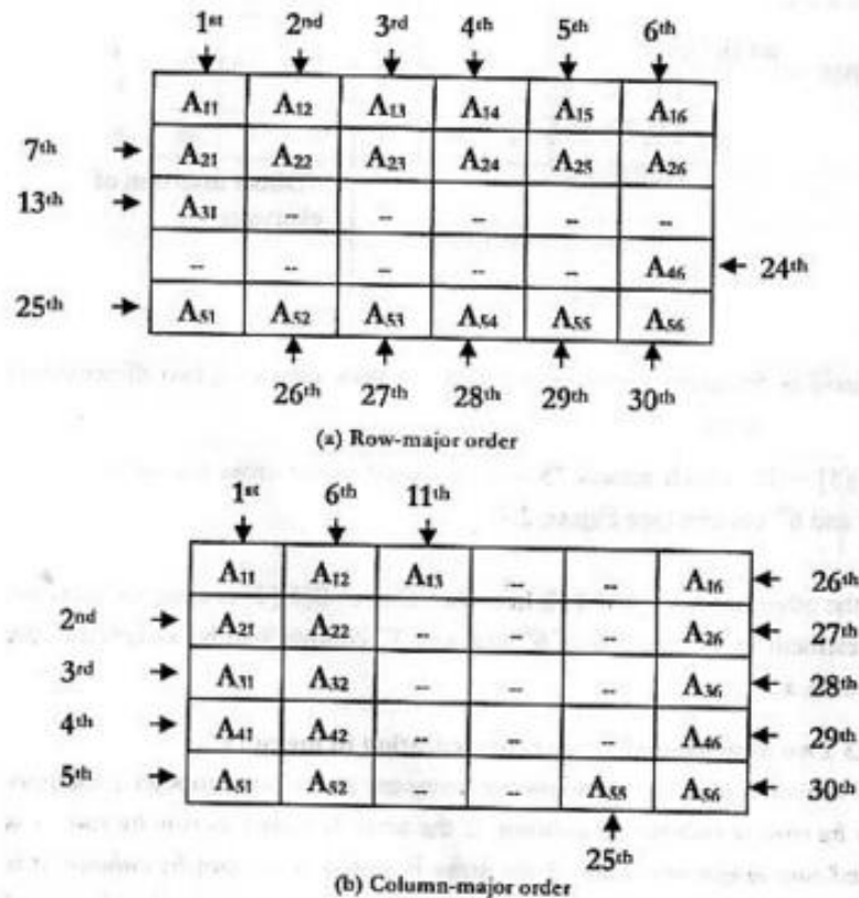
Figure-2.7: Pictorial view of two dimensional array representation in memory
