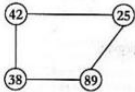
Undirected Graph
