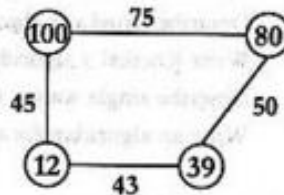
Connected Graph
