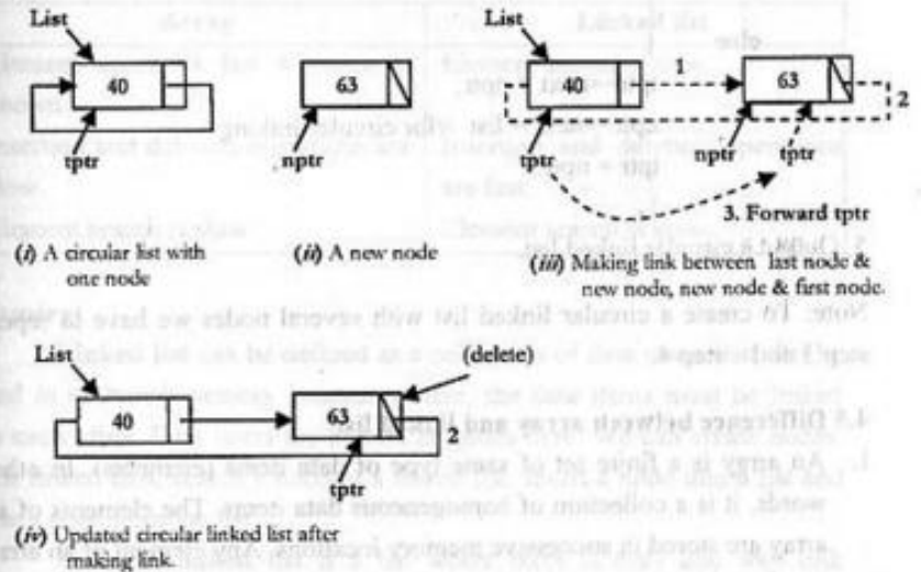
Figure-4.12: Creation of a circular linked list with more than one node
