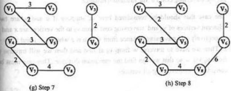
Figure-8.10: Pictorial view of the stages of the Kruskal's algorithm.
