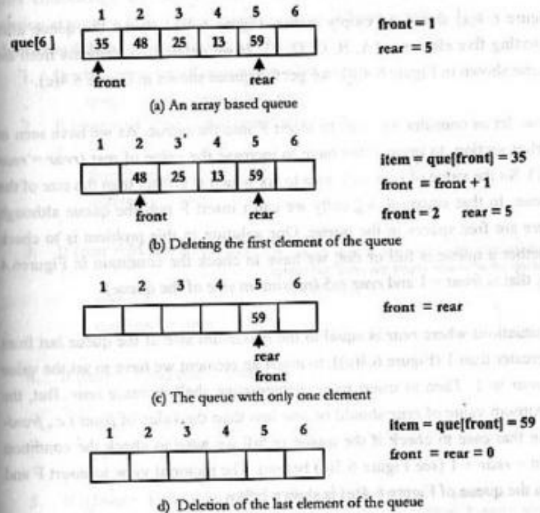
Figure-6.3: Deletion process of an array based queue (pictorial view)
