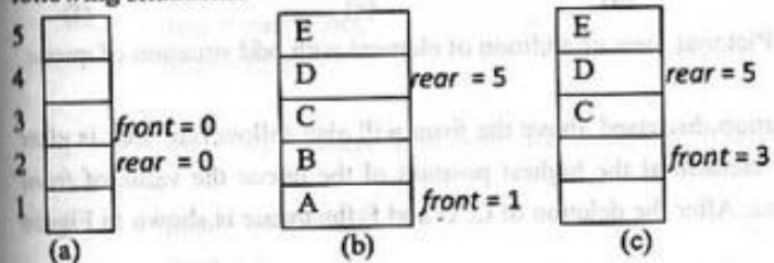
Figure-6.4: Pictorial view with odd situation of queue
