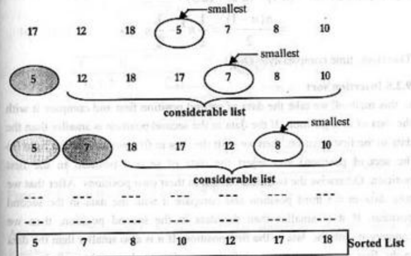
Figure-9.3: Pictorial view of selection sort
