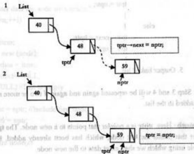
Figure-4.2: Addition of nodes to a linked list (pictorial view)
