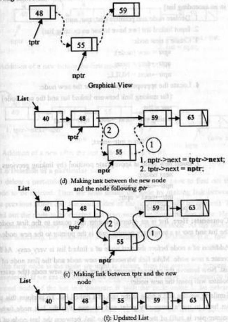
Figure-4.3: New node insertion in an existing list (pictorial view)
