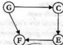
Directed Graph
