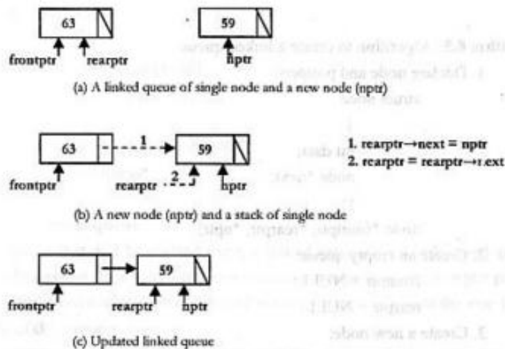
Figure-6.7: Pictorial view of linked queue (creation process)
